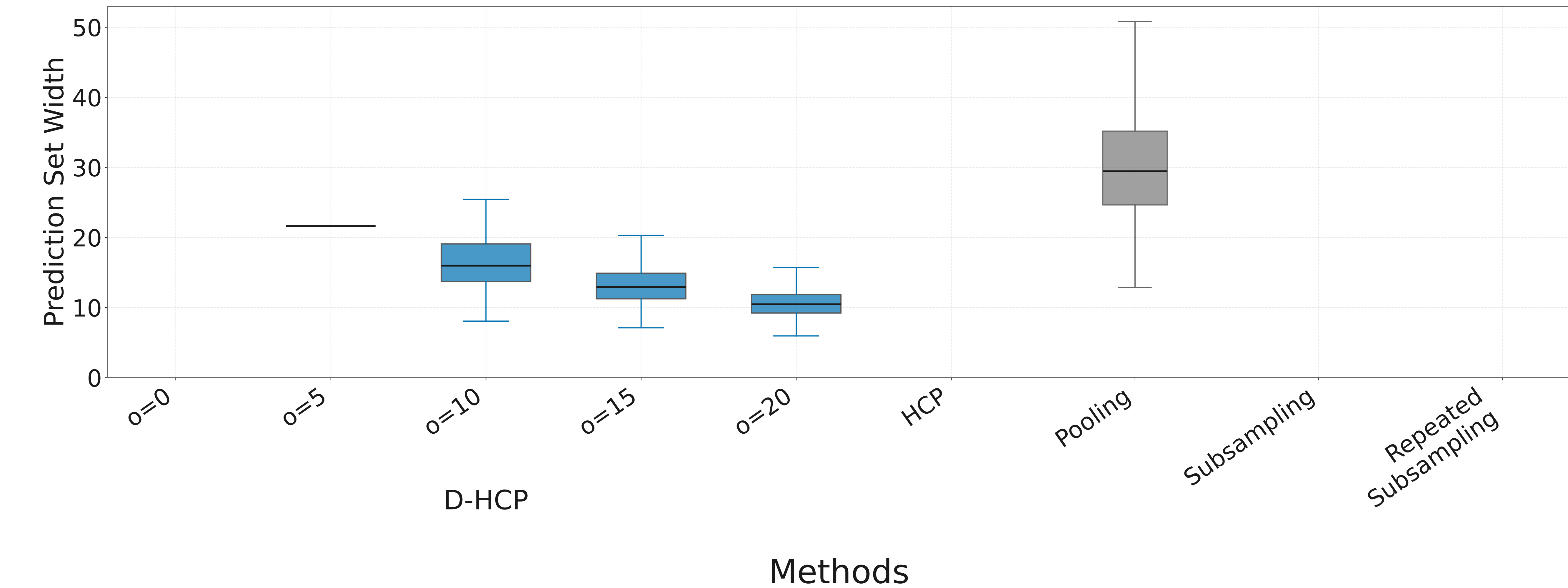
Poisson (RF): Prediction set width (all methods)
