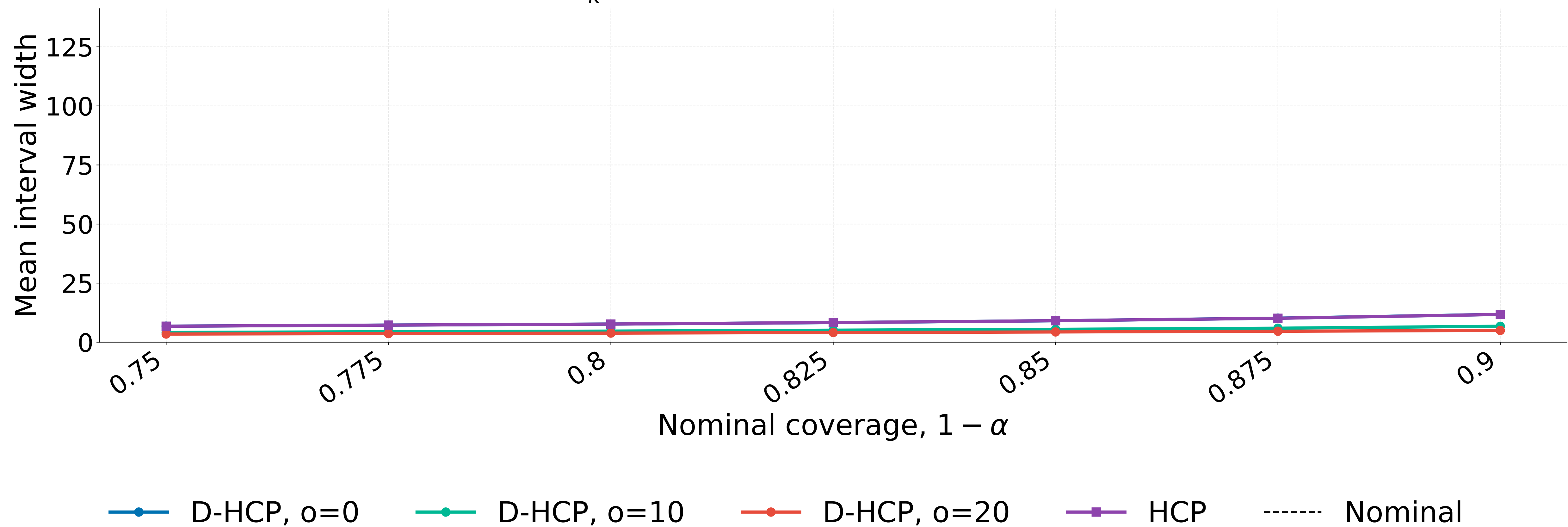
Fixed N_k = 21 : Width with standard-error bands
