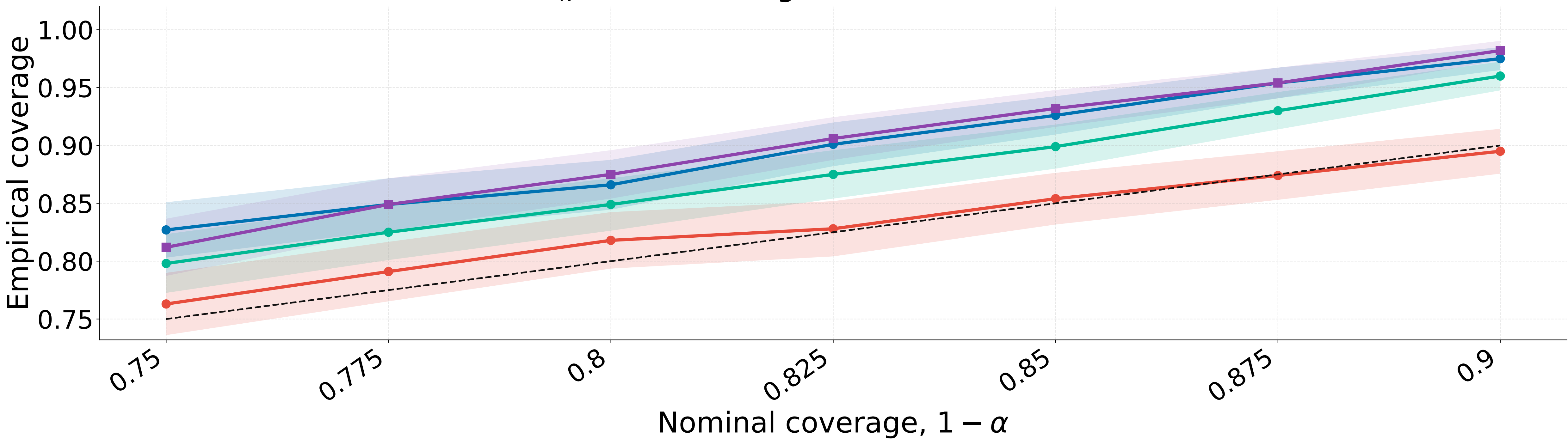
Fixed N_k = 21 : Coverage with standard-error bands
