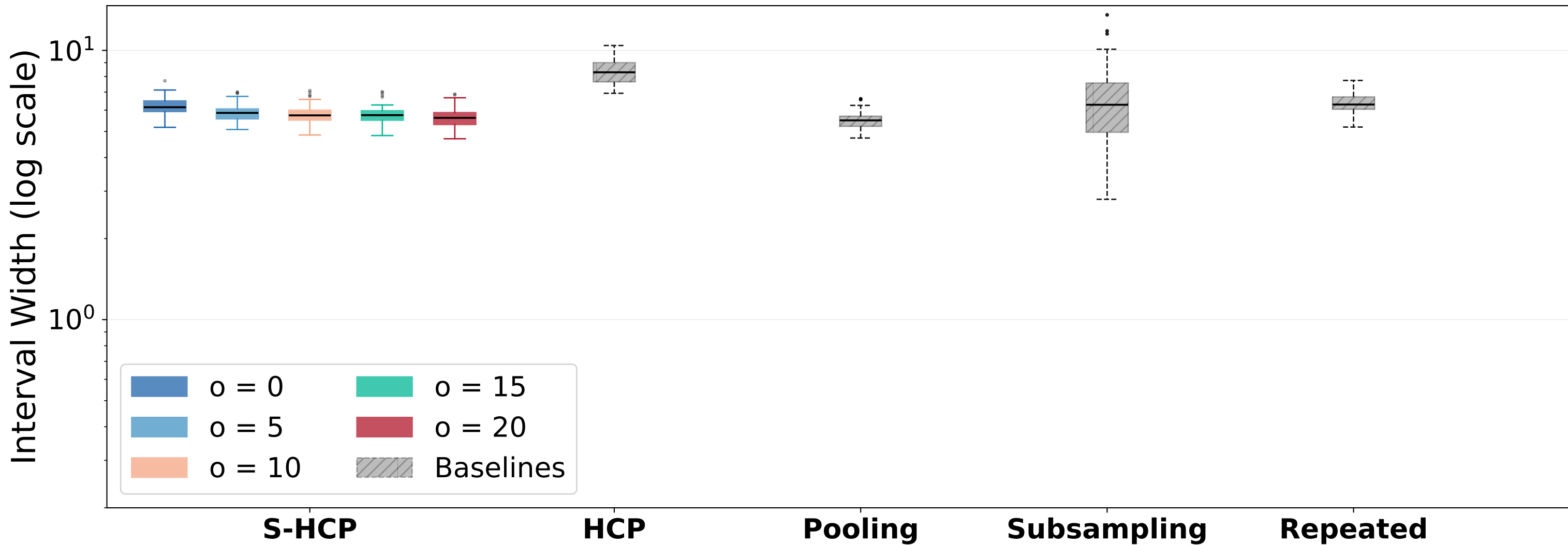
Interval Width (log scale) — Sample Focus — \lambda = 21
