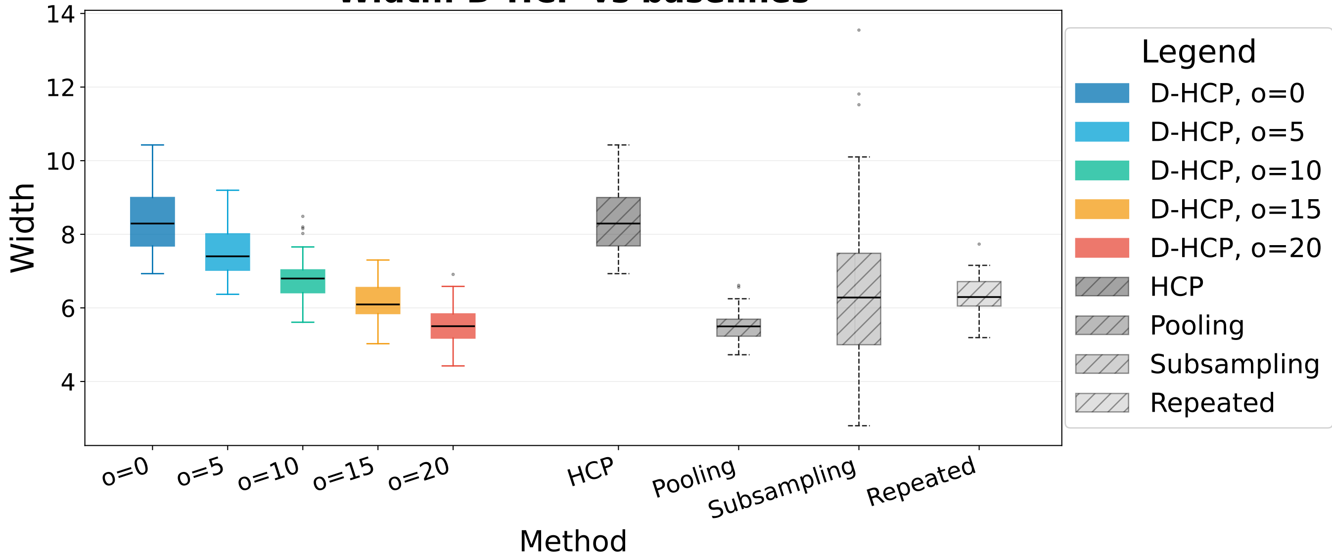
Width: D-HCP vs baselines
