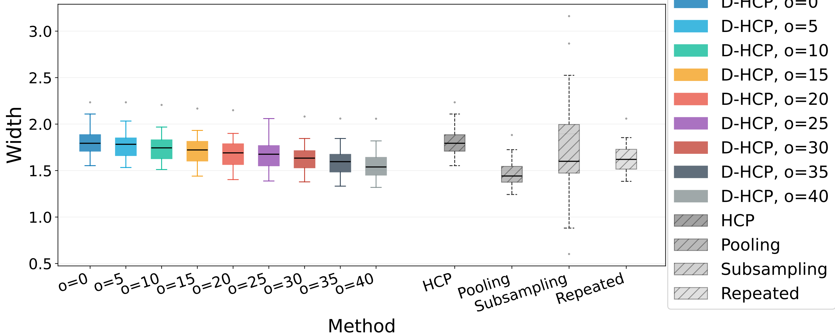
Width: D-HCP vs baselines
