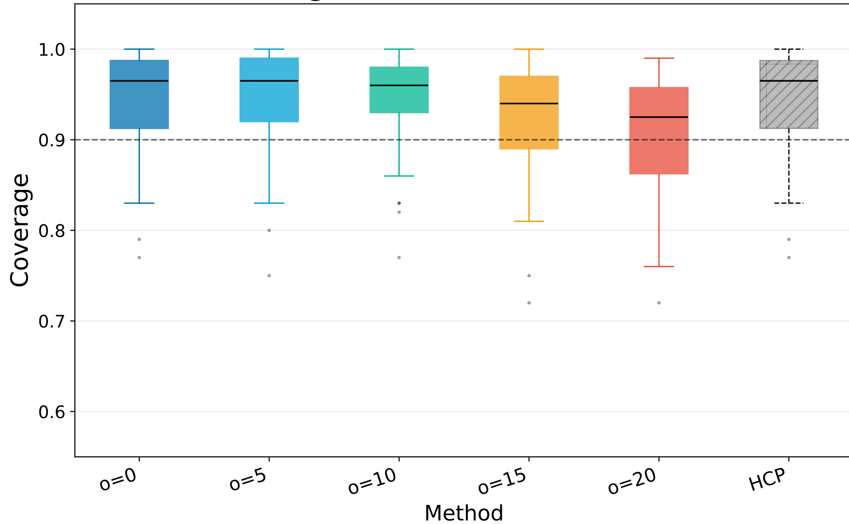
Coverage: Donor-HCP(within) vs HCP
