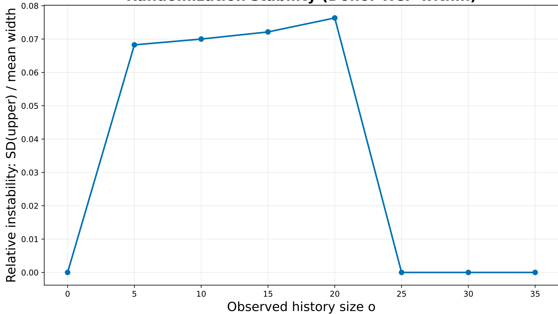
Randomization stability (Donor-HCP within)
