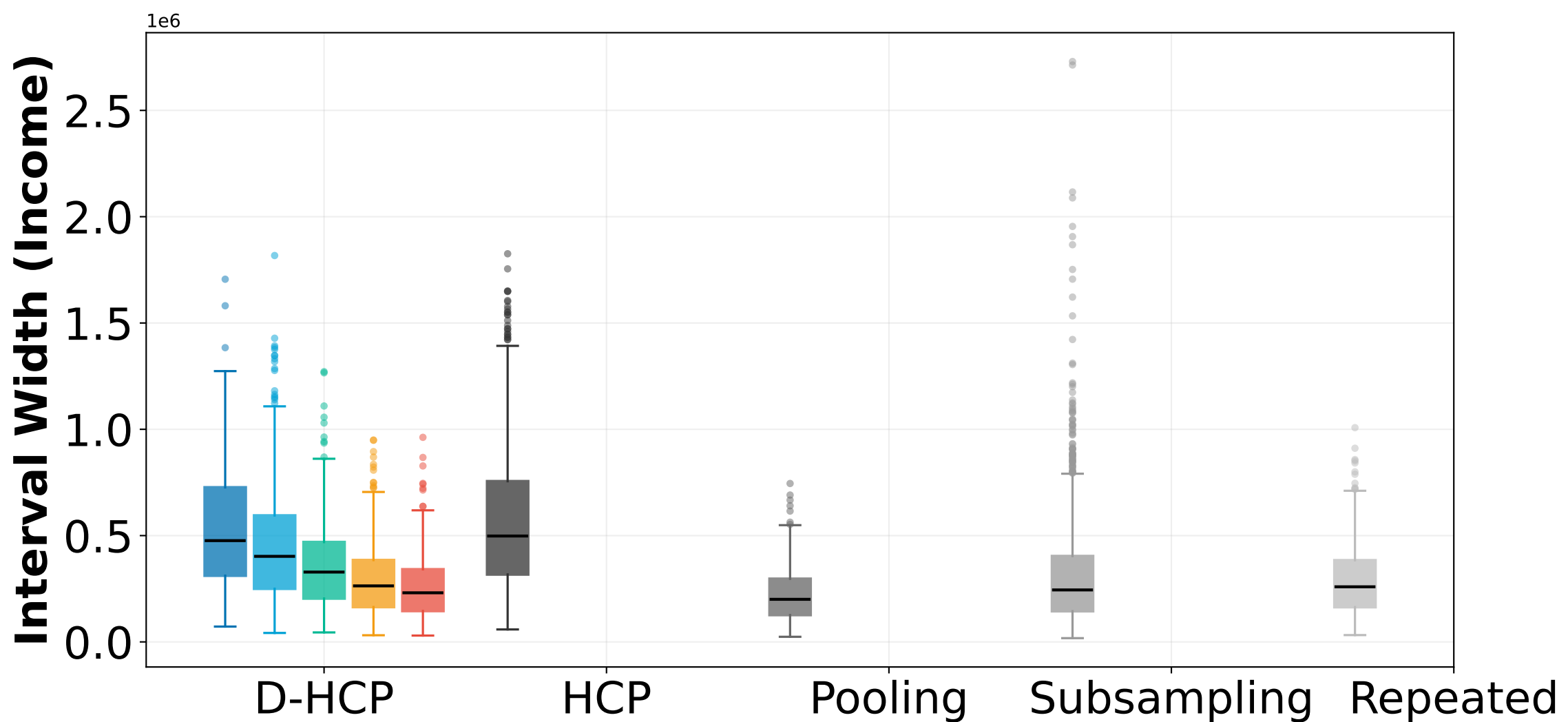
Interval Width: D-HCP vs Baselines (True Marginal)
