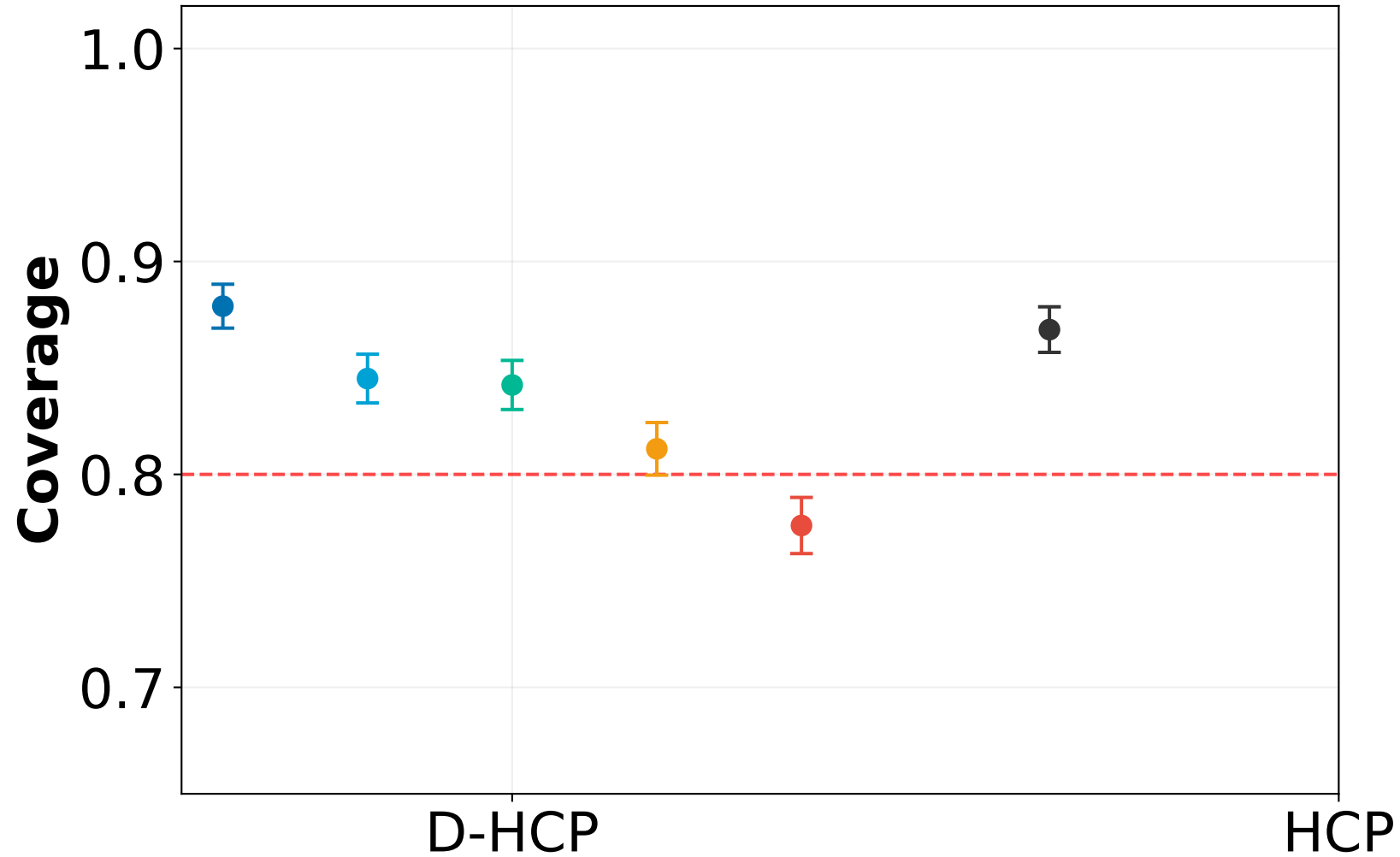
Coverage: D-HCP vs HCP (True Marginal)
