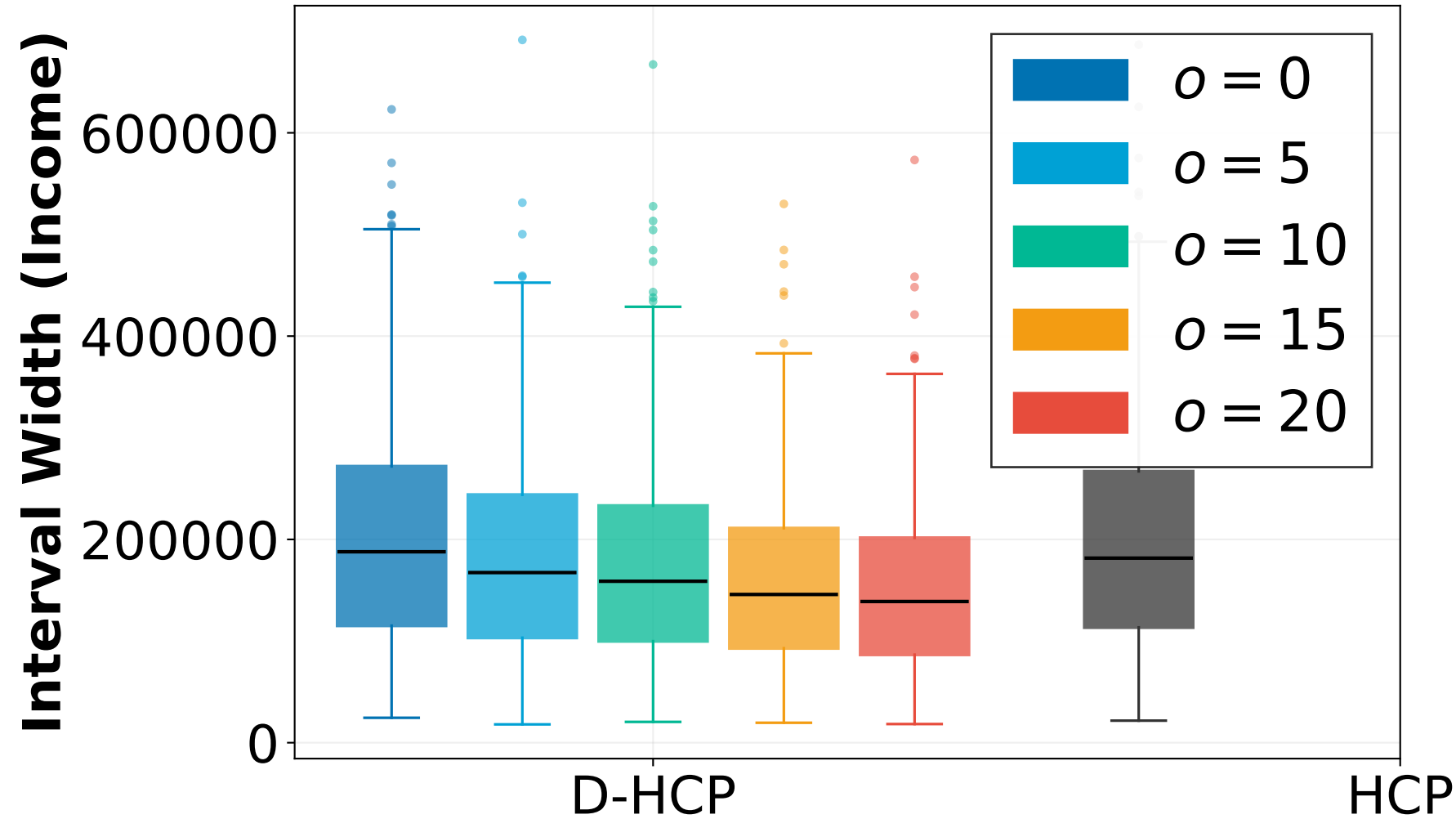
Interval Width: D-HCP vs HCP (True Marginal)
