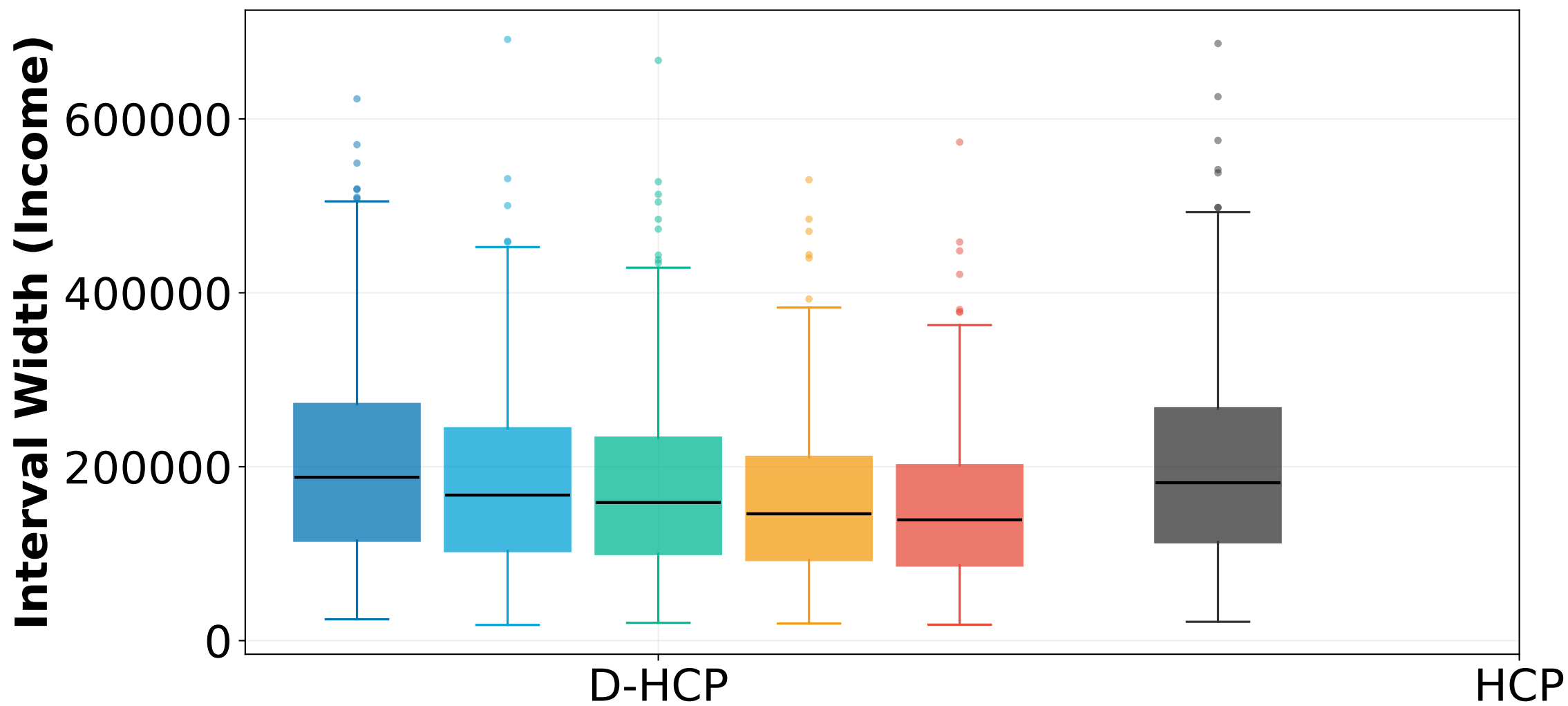
Interval Width: D-HCP vs HCP, All o (True Marginal)
