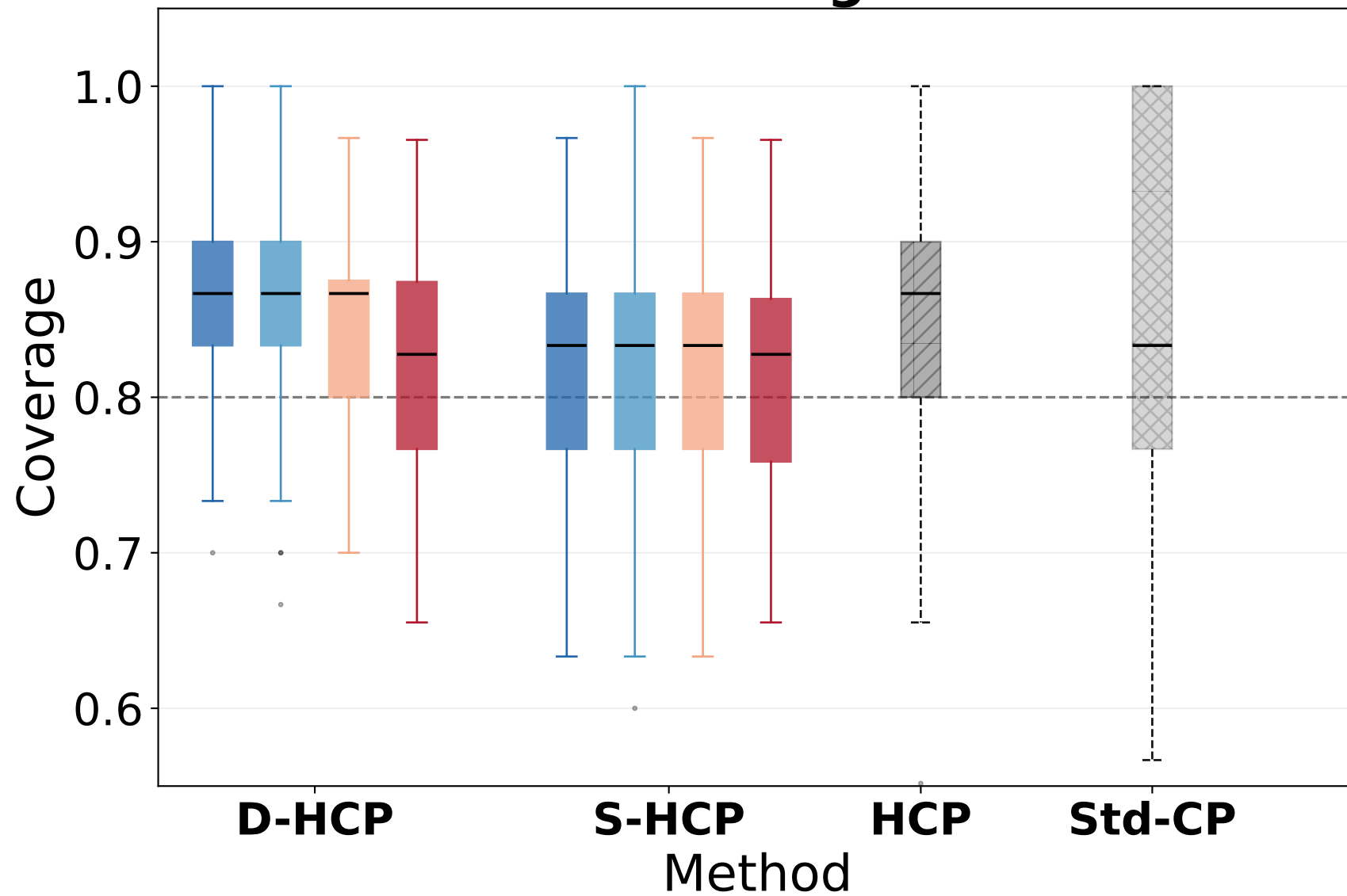
D-HCP / S-HCP vs HCP / Std-CP - ACS (CA fixed PUMA groups, alpha=0.2) Coverage Interval Width (income units, 90th pct clipped)
