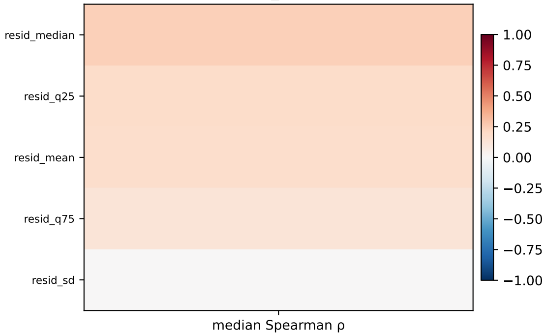
Median Spearman \rho : N_j vs residual summaries
