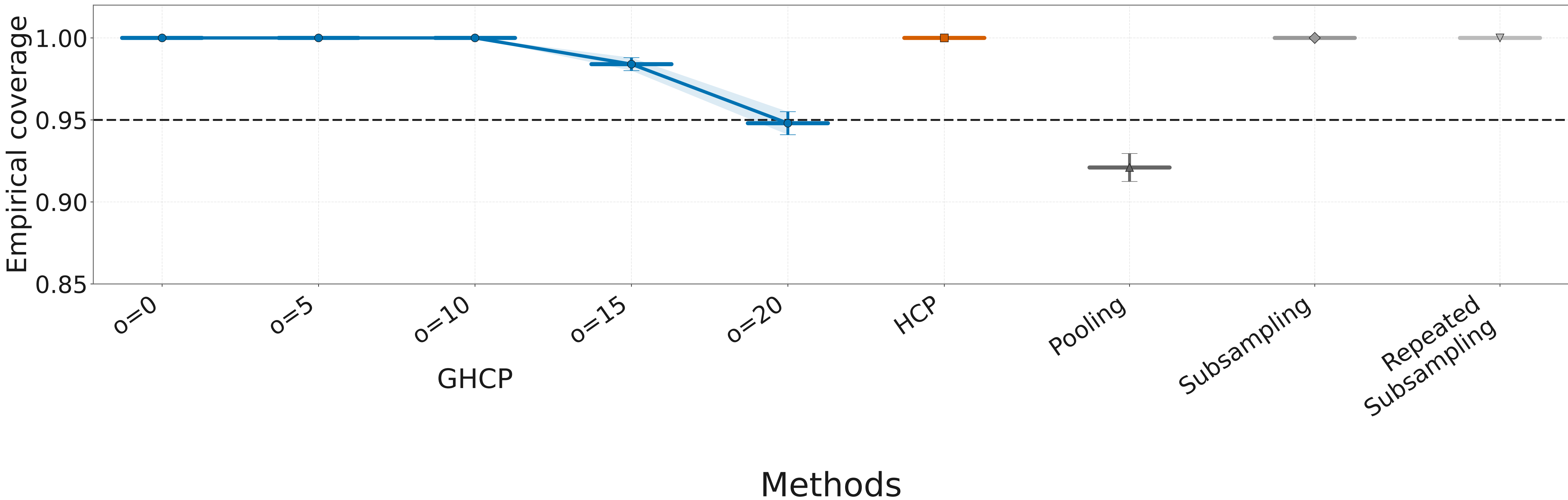
Fixed N_k = 21 (RF): Coverage (all methods)
