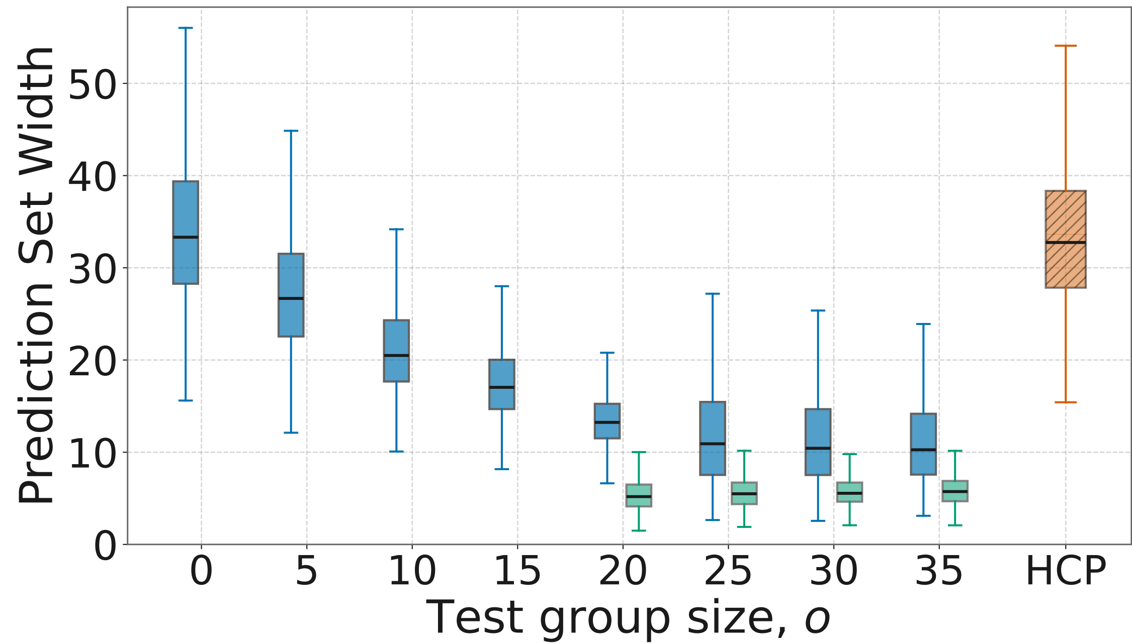
Prediction Set Width
