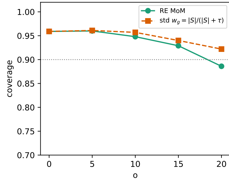
\gamma = 5, \alpha = 0.1 coverage
