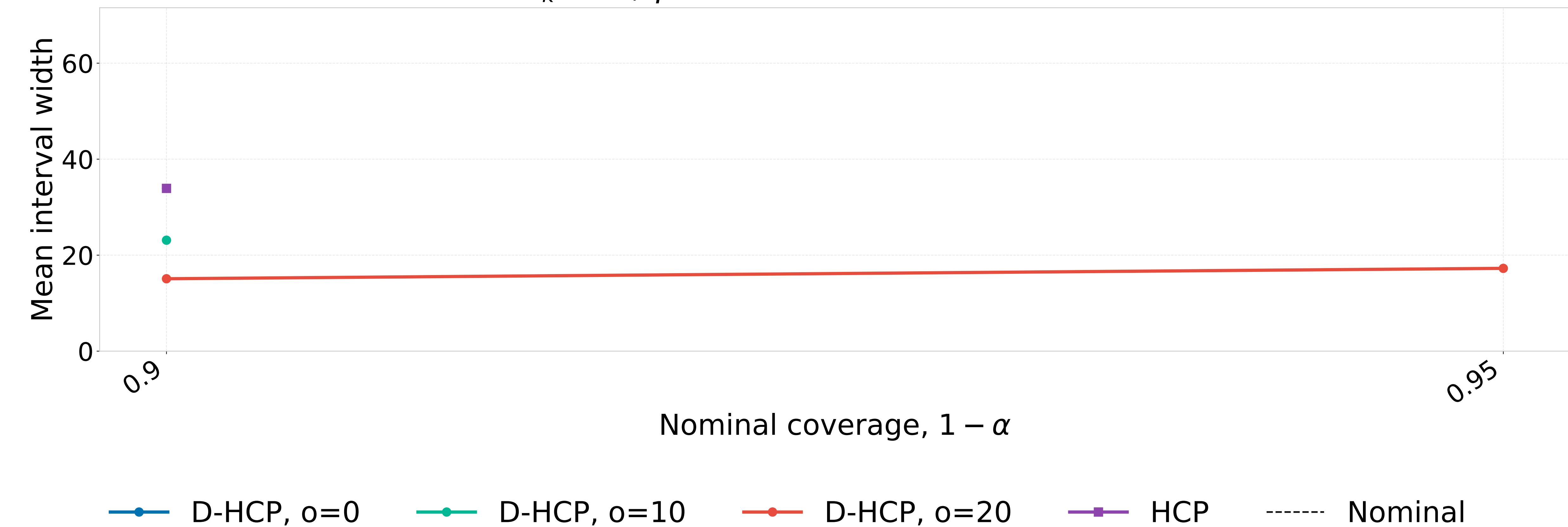
Fixed N_k = 21 , \gamma = 5 : Width with standard-error bands
