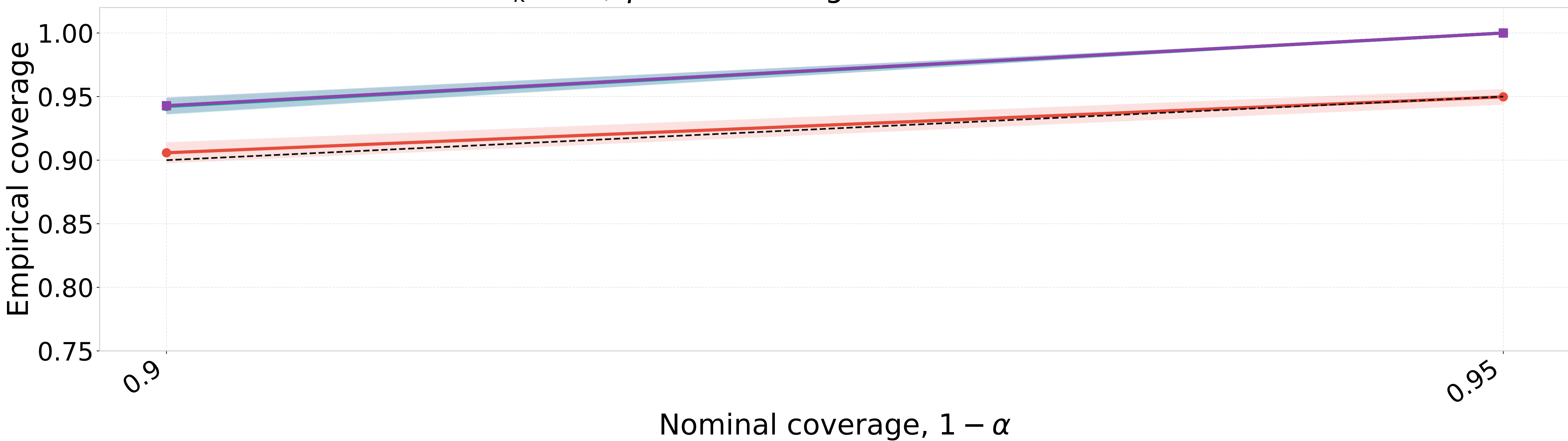
Fixed N_k = 21 , \gamma = 5 : Coverage with standard-error bands
