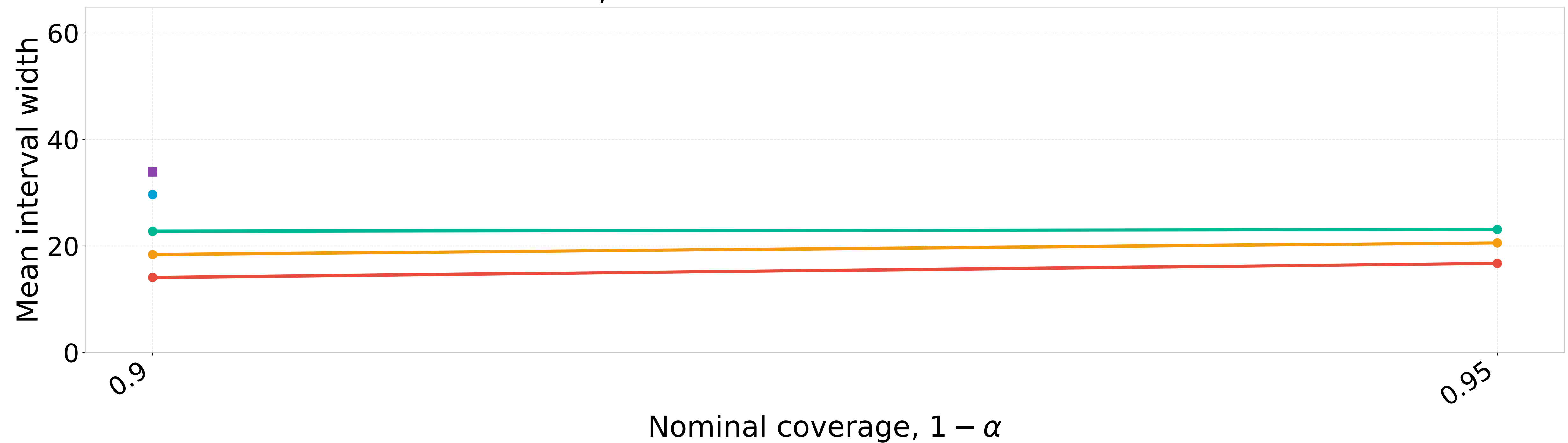
Poisson, \gamma = 5 : Width with standard-error bands
