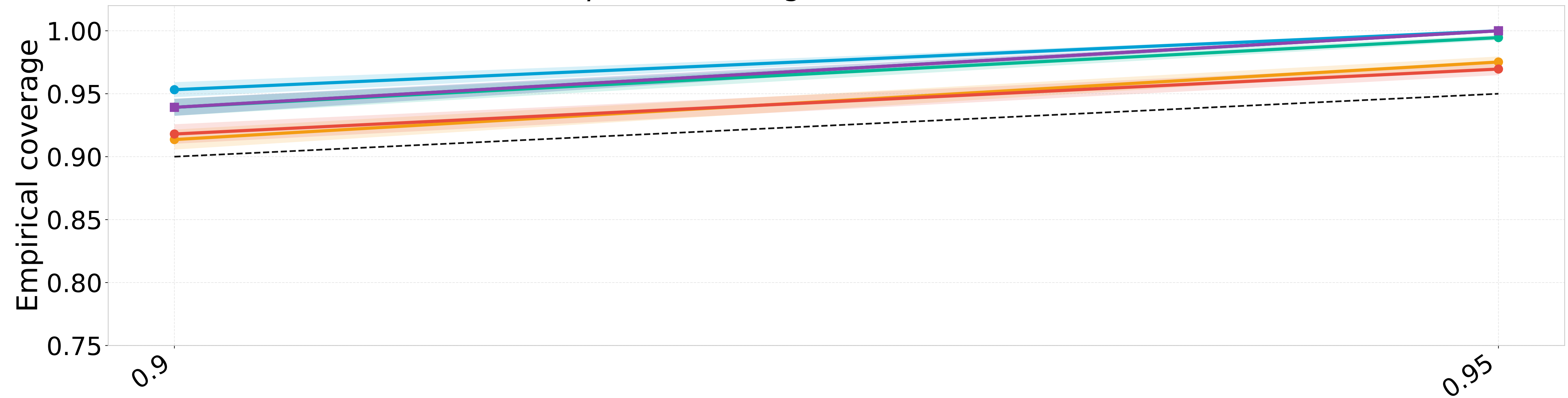
Poisson, \gamma = 5 : Coverage with standard-error bands
