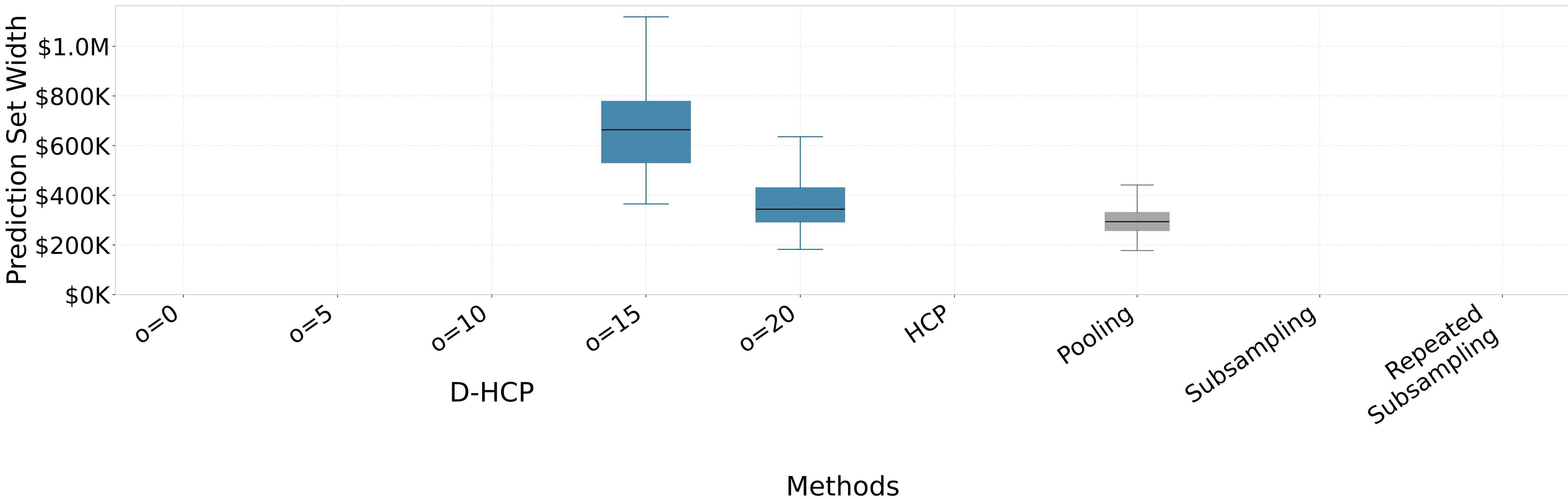
ACS: Prediction set width (all methods)
