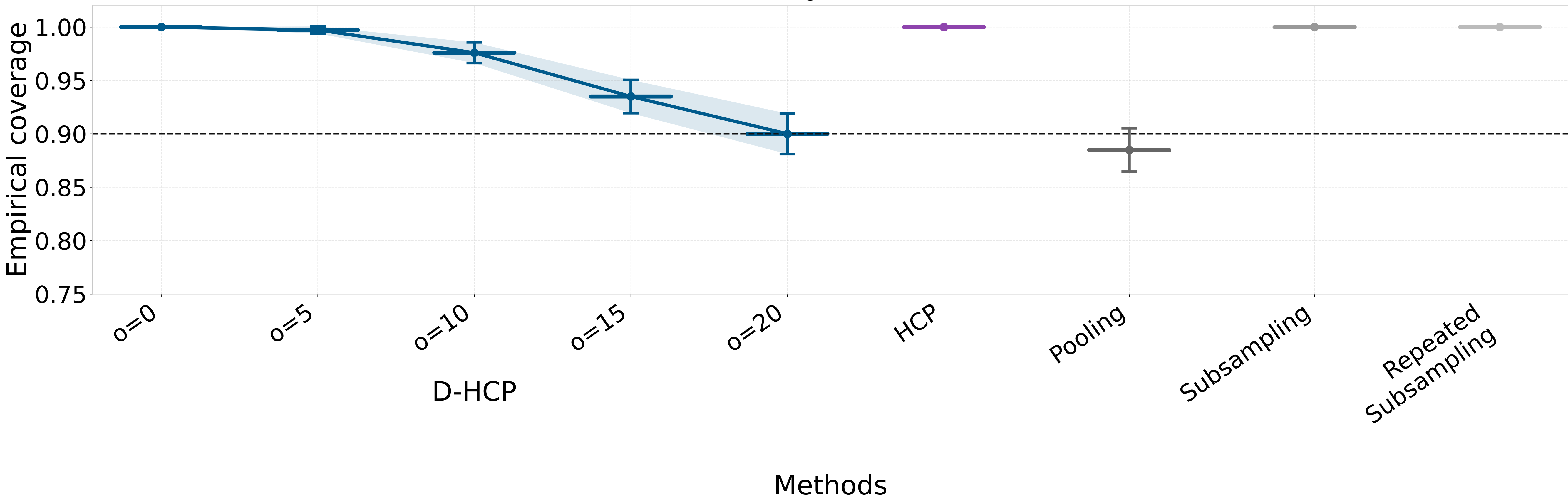
ACS: Coverage (all methods)
