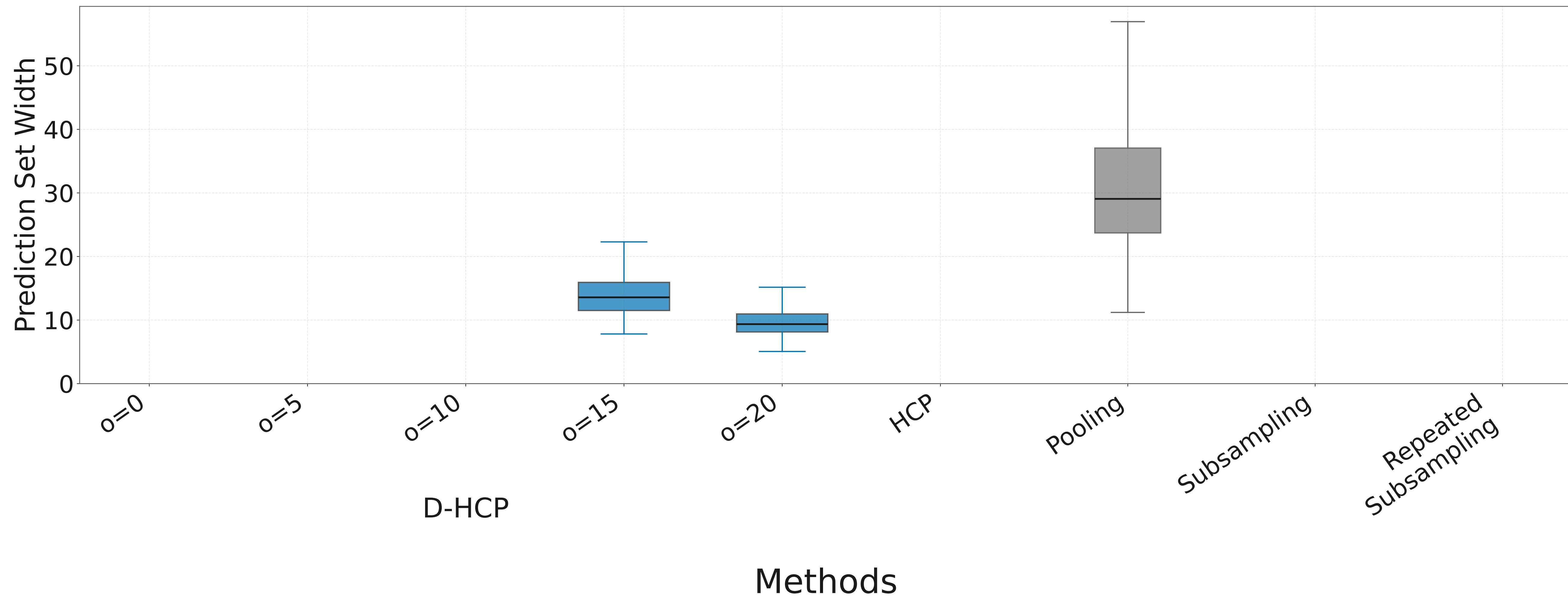
Fixed N_k = 21 : Prediction set width (all methods)
