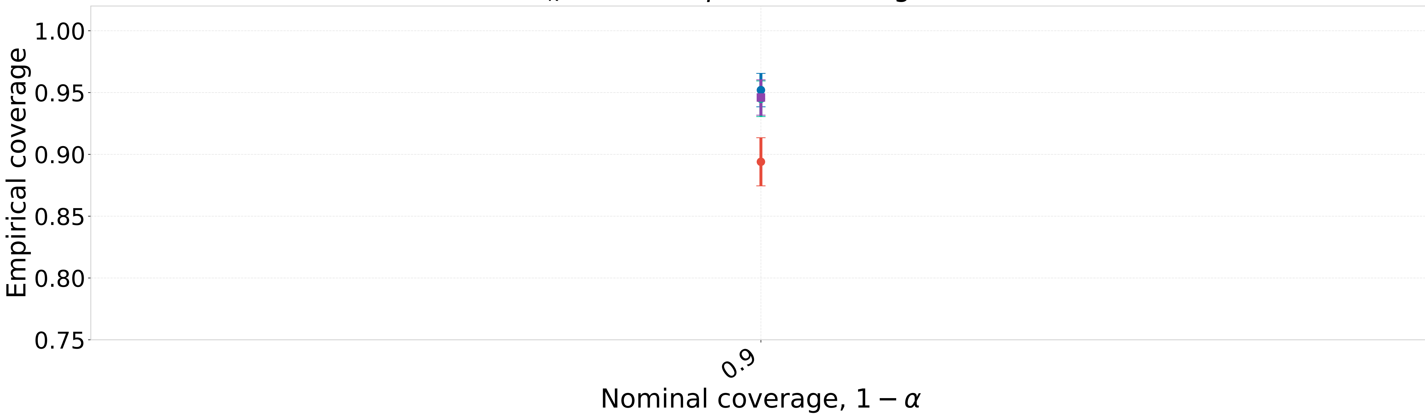
Fixed N_k = 21 (RF, \gamma = 5 ): coverage over 1 - \alpha
