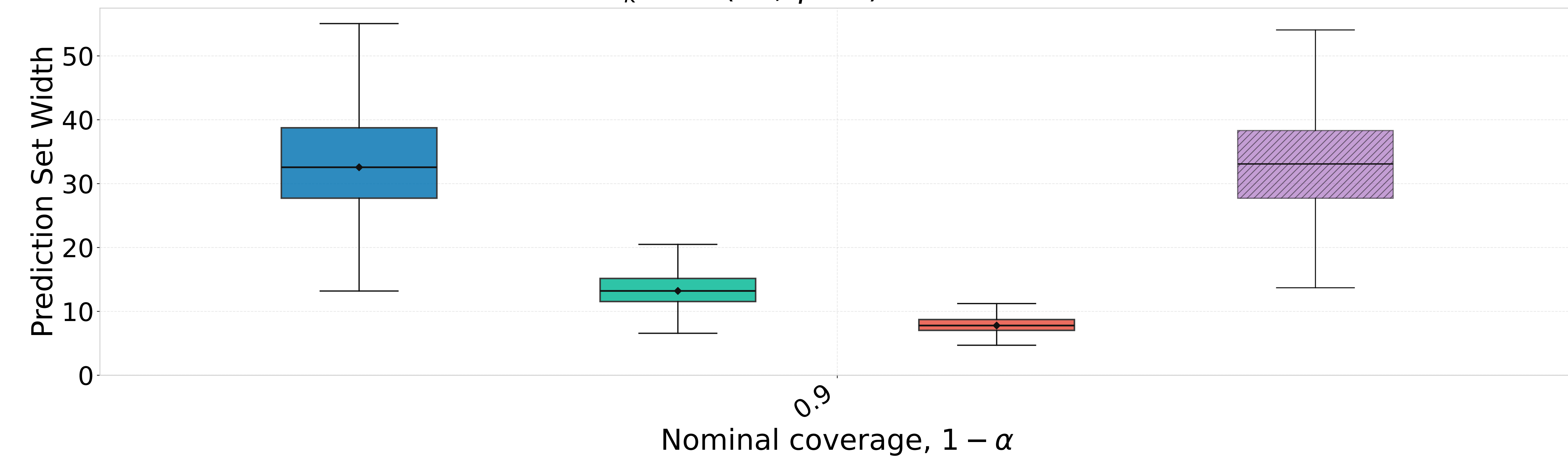
Fixed N_k = 21 (RF, \gamma = 5 ): widths over 1 - \alpha
