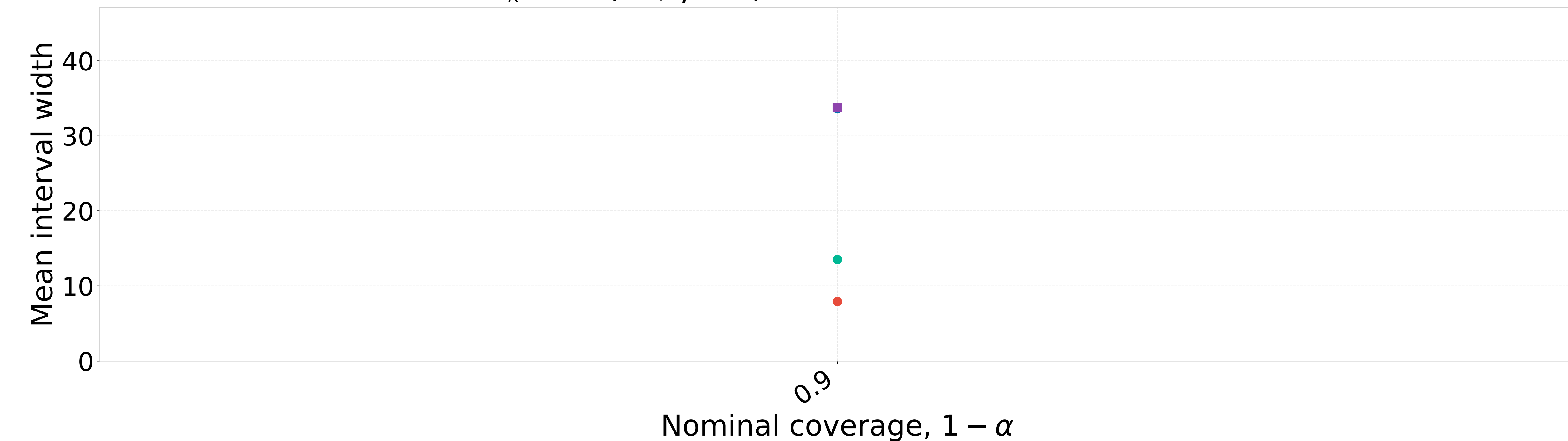
Fixed N_k = 21 (RF, \gamma = 5 ): Width with standard-error bands
