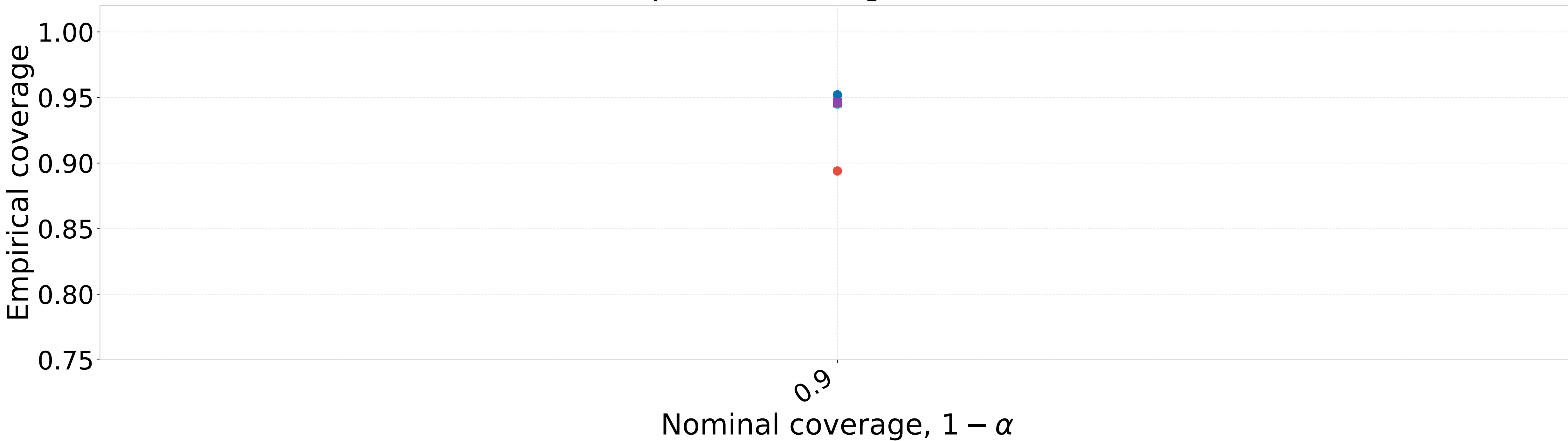
Fixed N_k = 21 (RF, \gamma = 5 ): Coverage with standard-error bands
