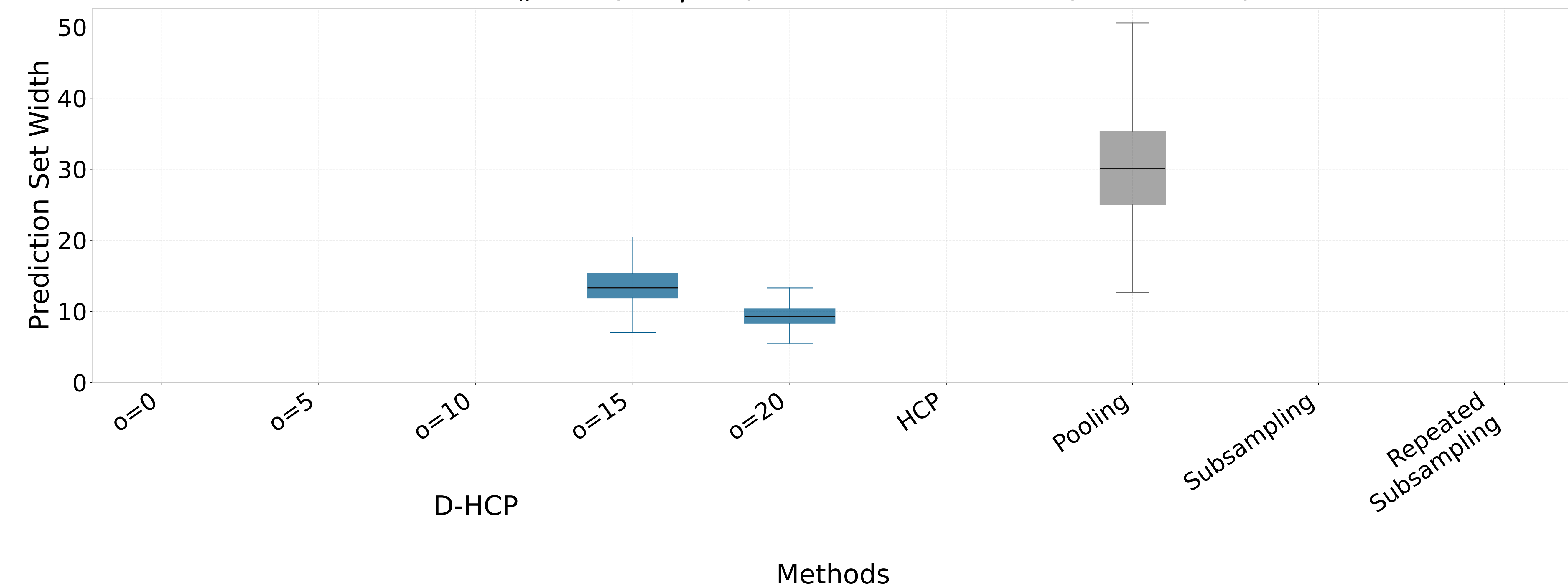
Fixed N_k = 21 (RF, \gamma = 5 ): Prediction set width (all methods)
