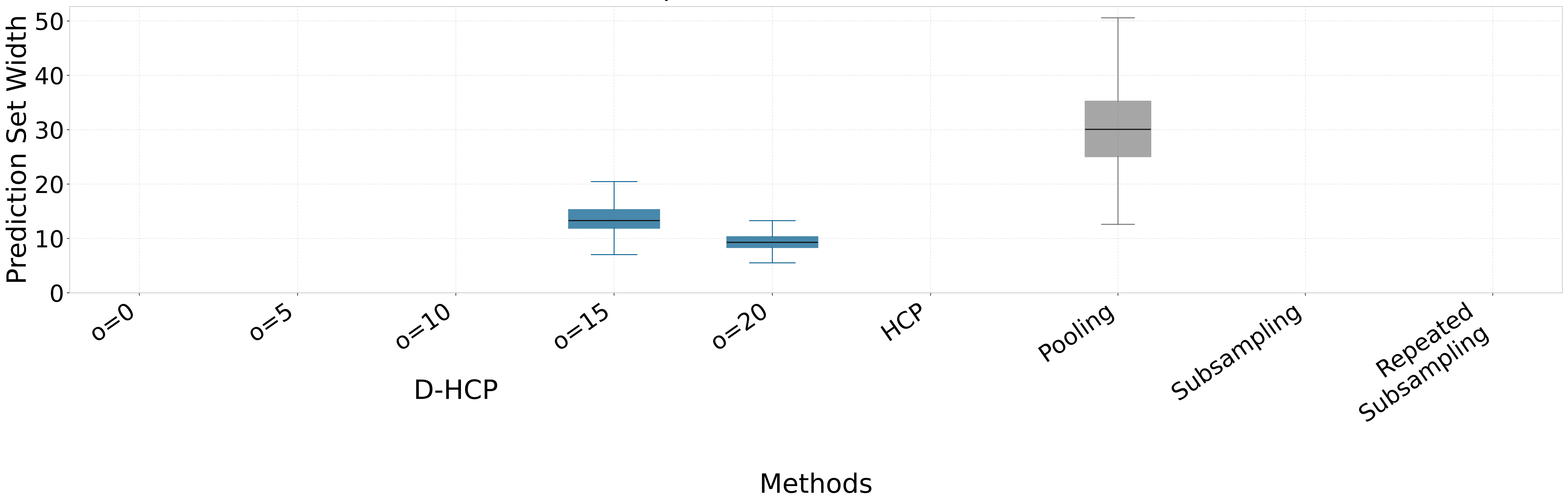
Fixed N_k = 21 (RF, \gamma = 5 ): Prediction set width (all methods)
