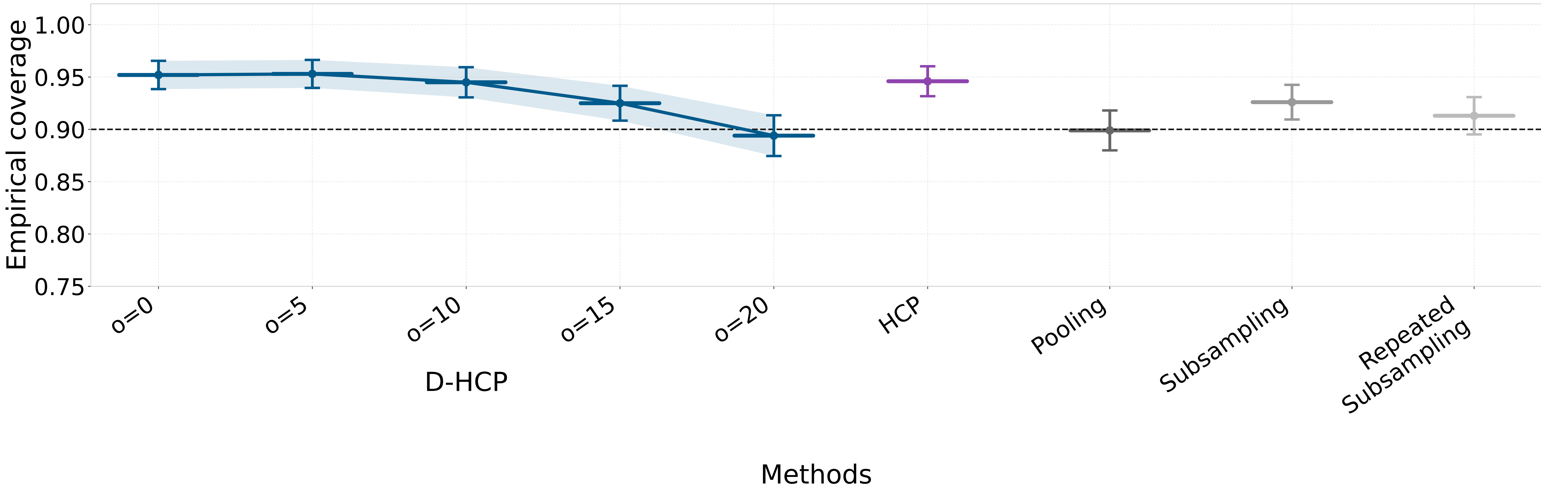
Fixed N_k = 21 (RF, \gamma = 5 ): Coverage (all methods)
