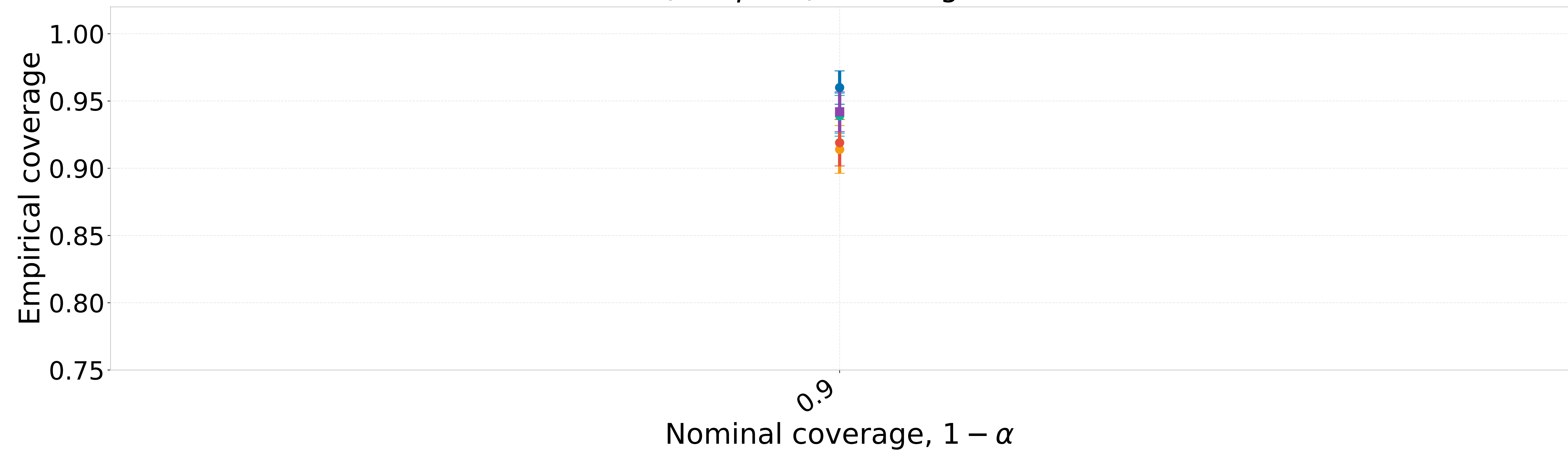
Poisson (RF, \gamma = 5 ): coverage over 1 - \alpha
