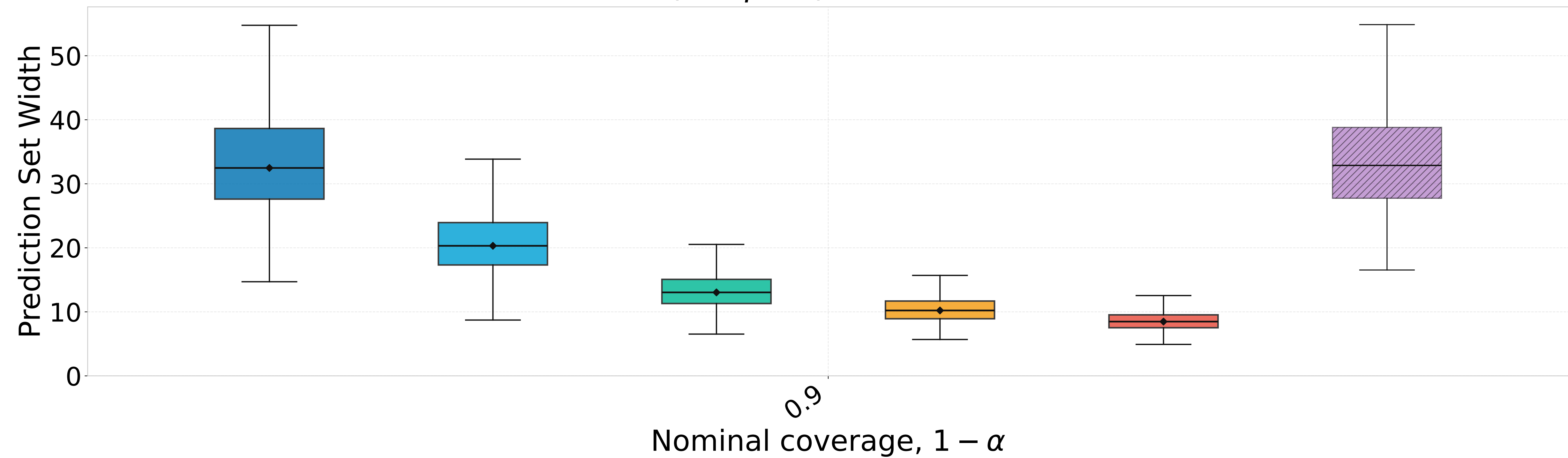
Poisson (RF, \gamma = 5 ): widths over 1 - \alpha
