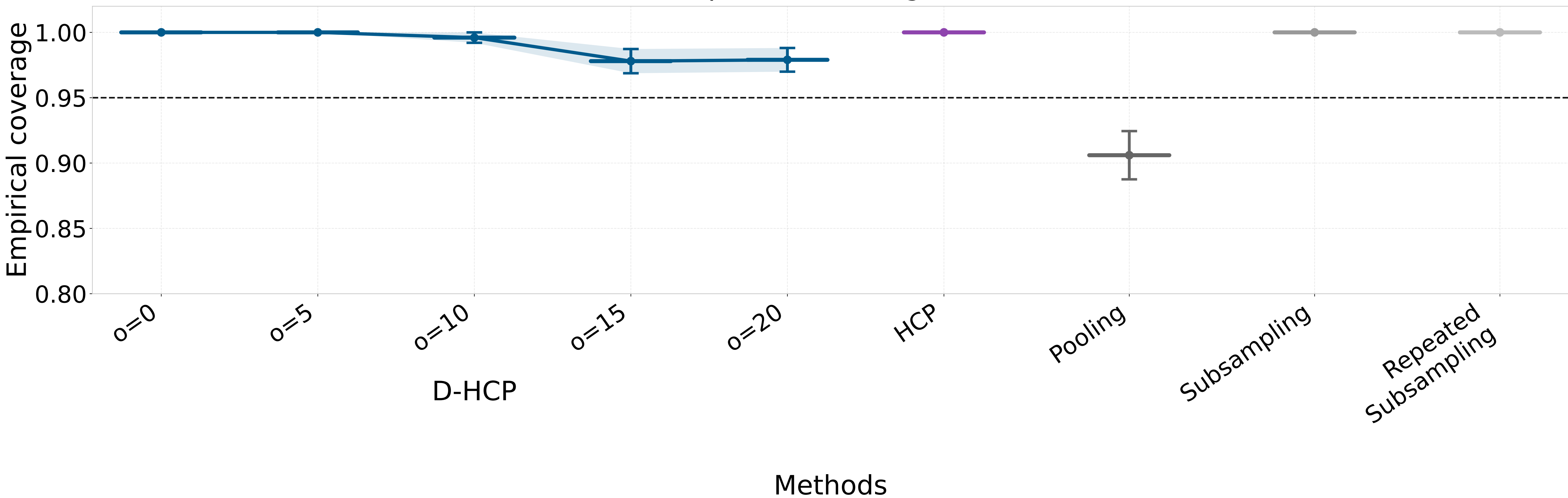
Poisson (RF, \gamma = 5 ): Coverage (all methods)
