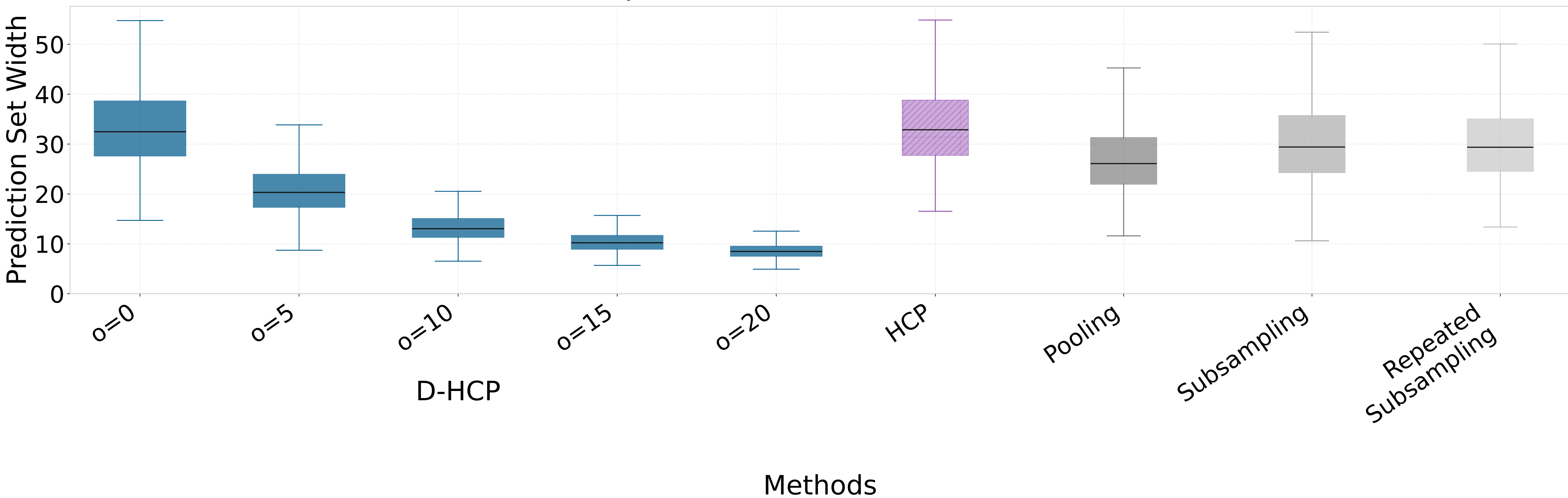
Poisson (RF, \gamma = 5 ): Prediction set width (all methods)
