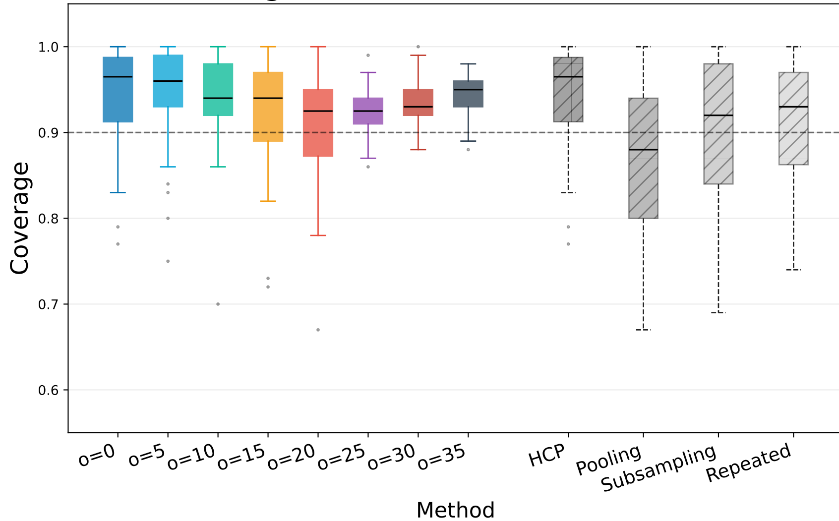
Coverage: Donor-HCP(within) vs baselines
