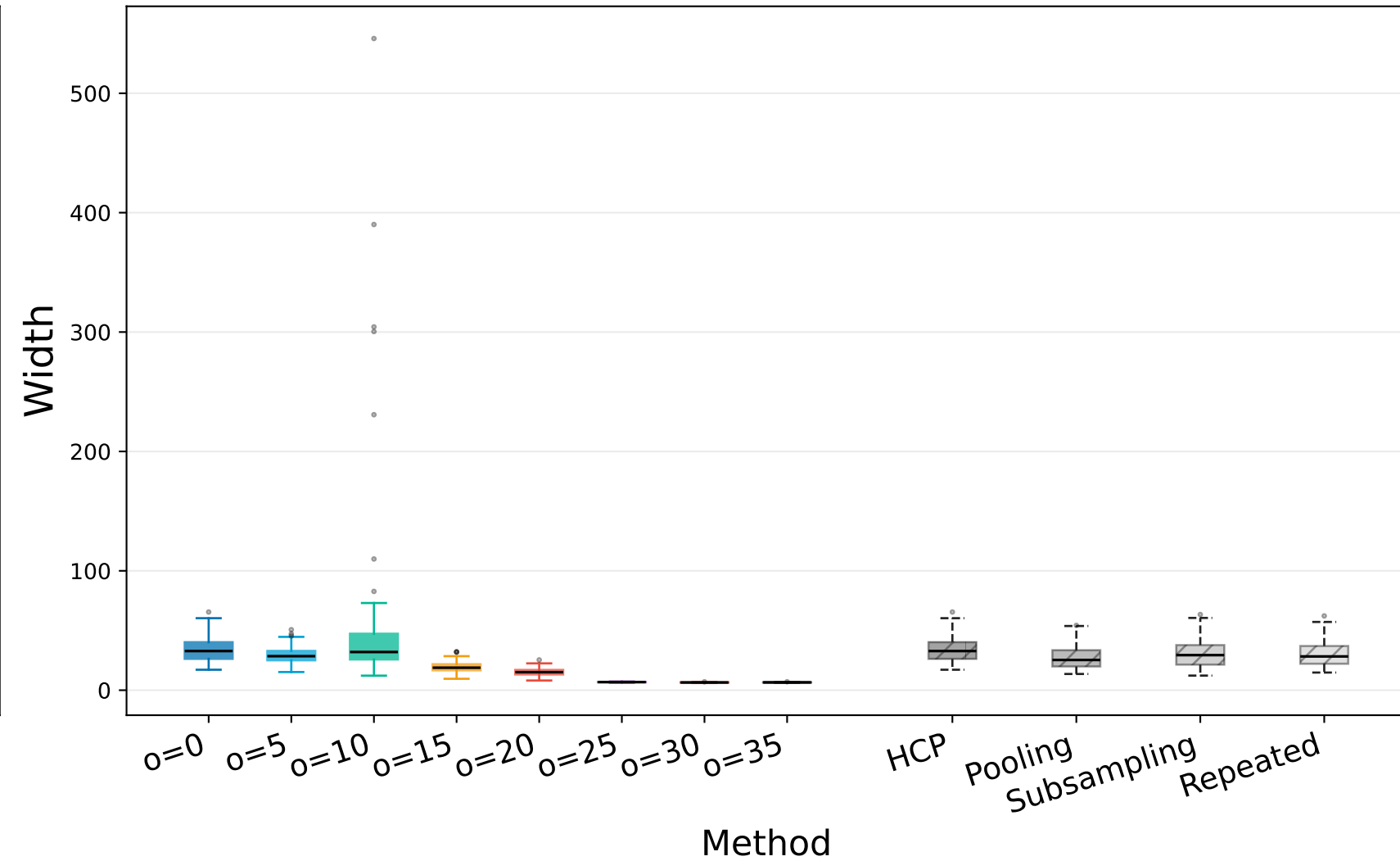
Width: Donor-HCP(within) vs baselines
