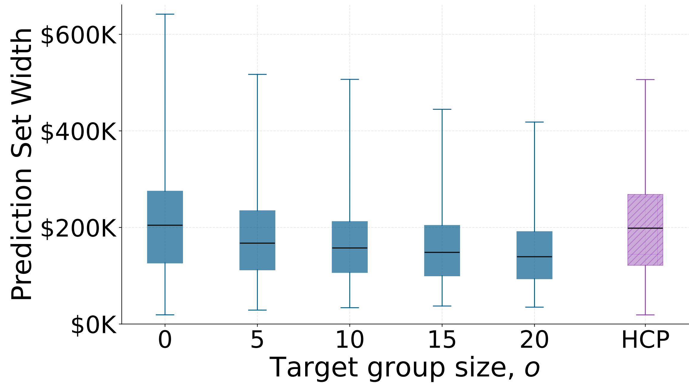
Prediction Set Width
