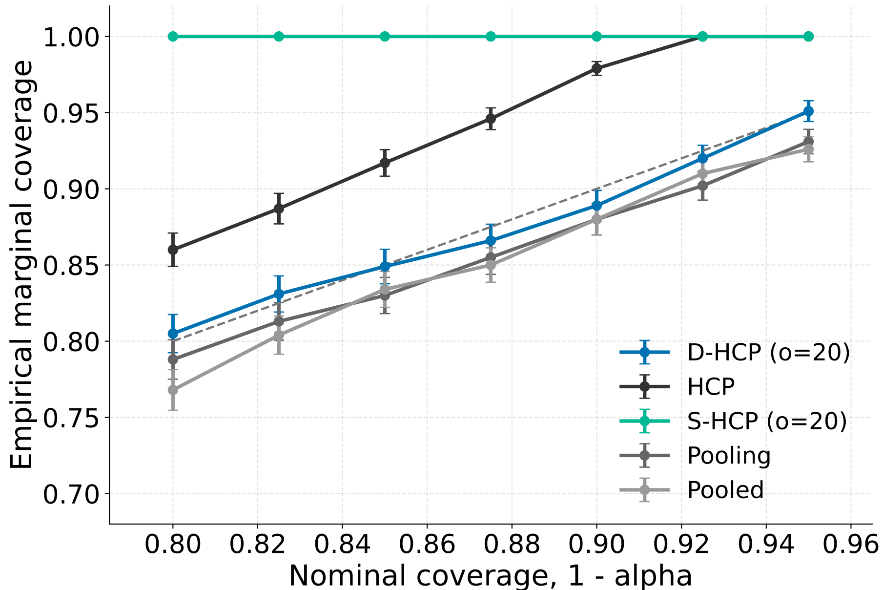
ACS true marginal coverage by method
