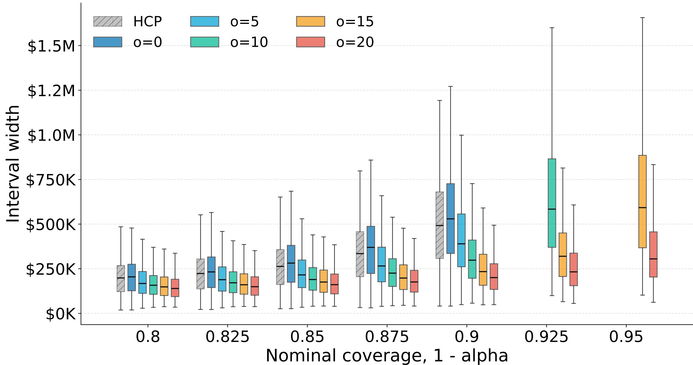
ACS true marginal width distributions
