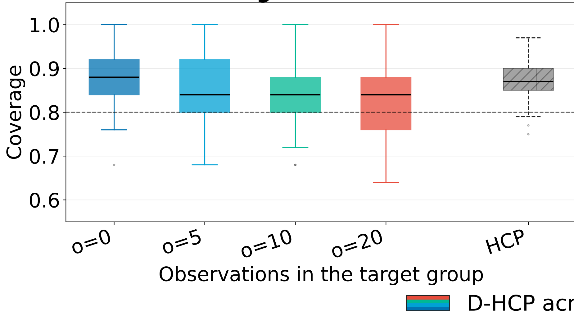
Coverage: D-HCP vs HCP
