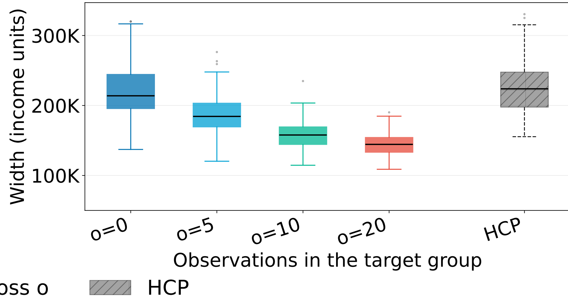
Width: D-HCP vs HCP
