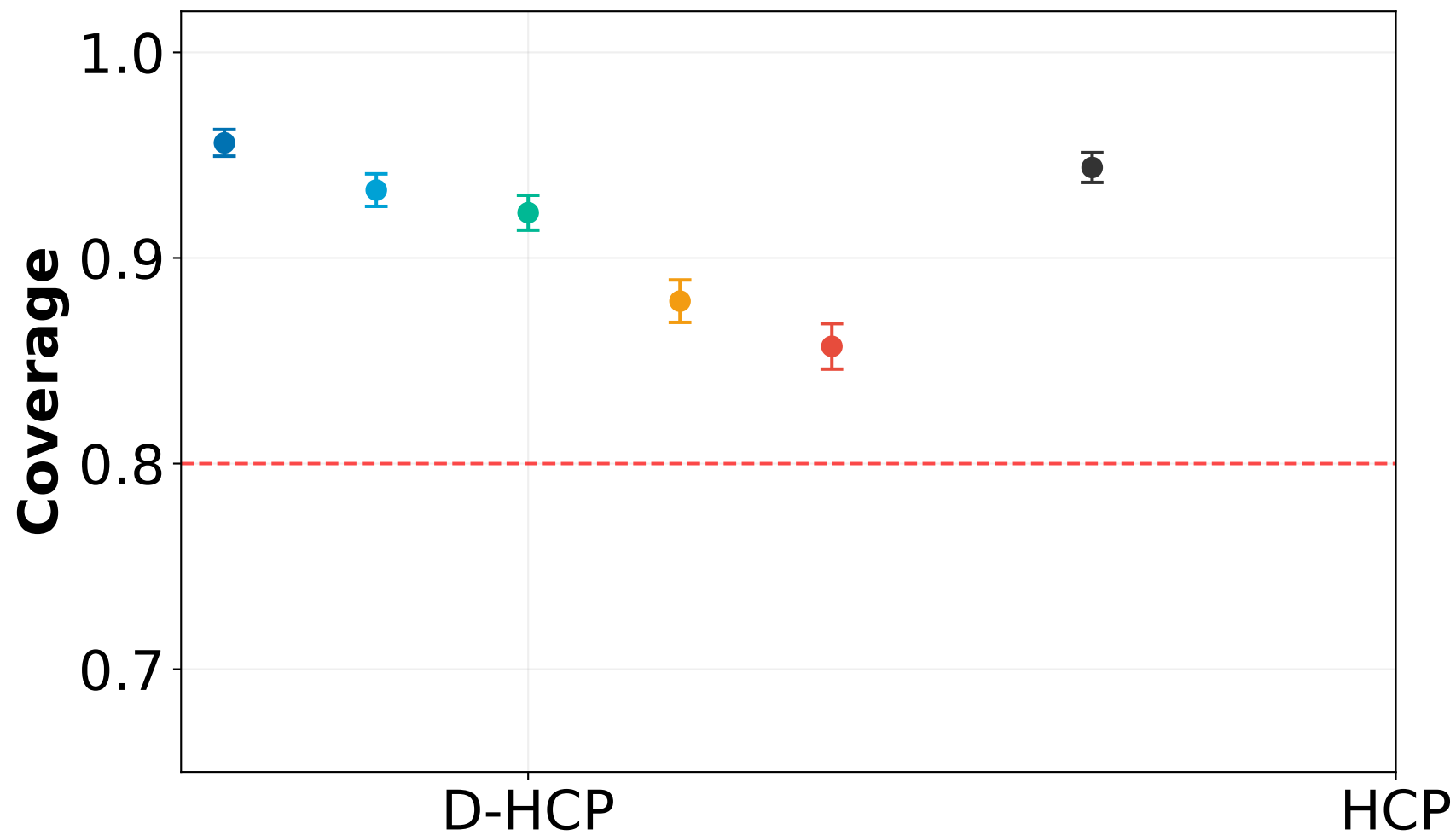
Coverage: D-HCP vs HCP (True Marginal) Interval Width: D-HCP vs HCP (True Marginal)
