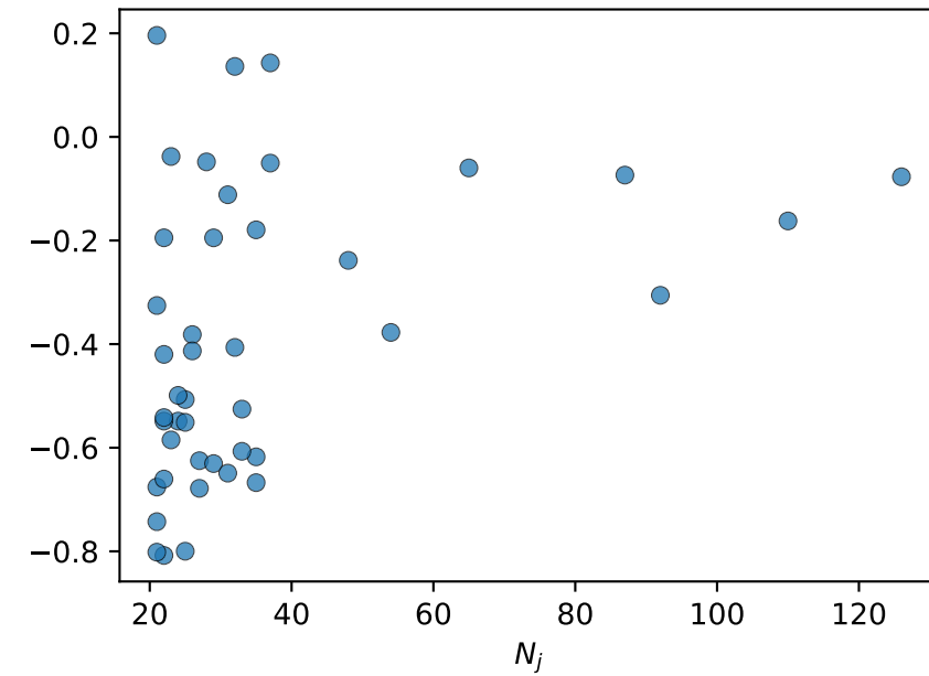
resid_q25 Spearman \rho=0.42
