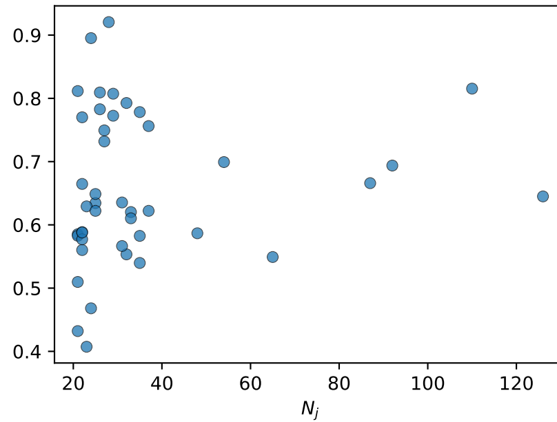
resid_sd Spearman \rho=0.22
