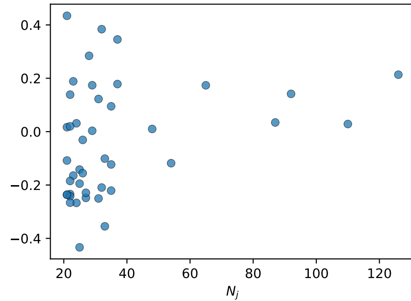
resid_mean Spearman \rho=0.33
