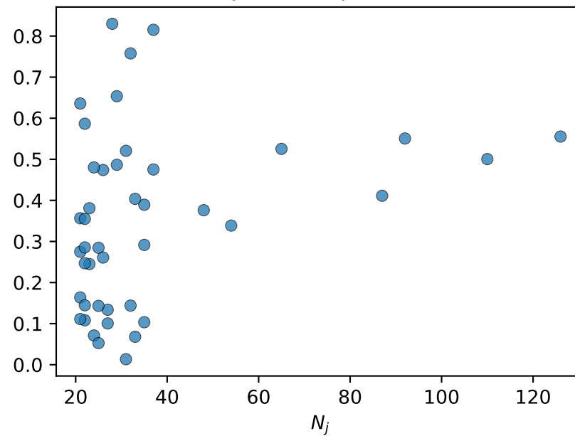
resid_q75 Spearman \rho=0.32
