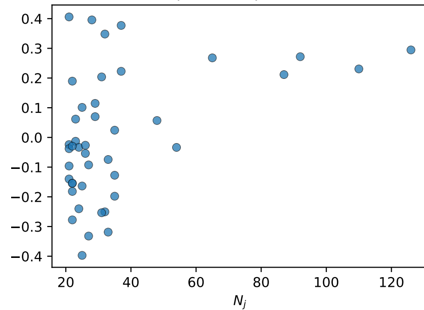
resid_median Spearman \rho=0.33
