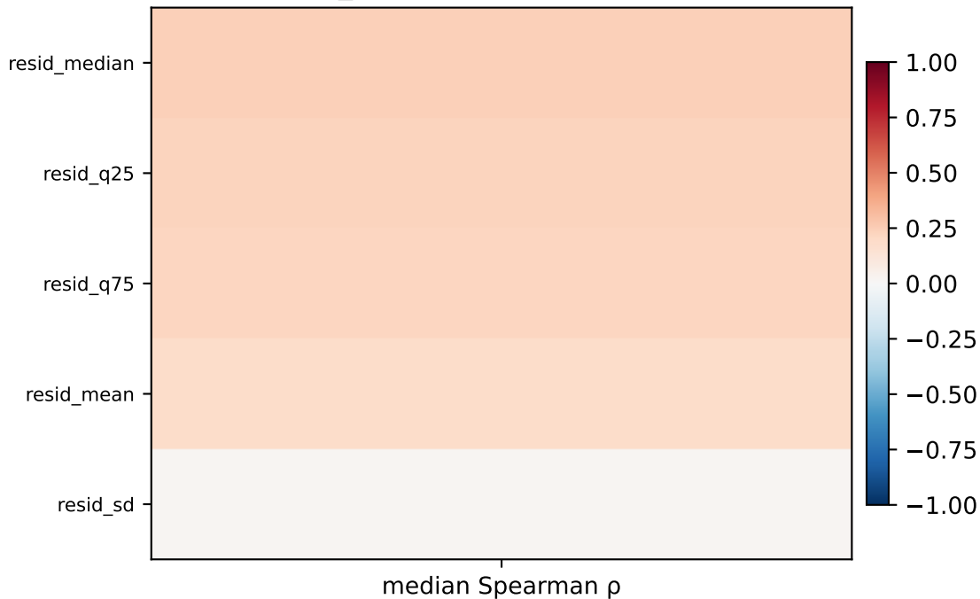
Median Spearman \rho : N_j vs residual summaries (across subsamples)
