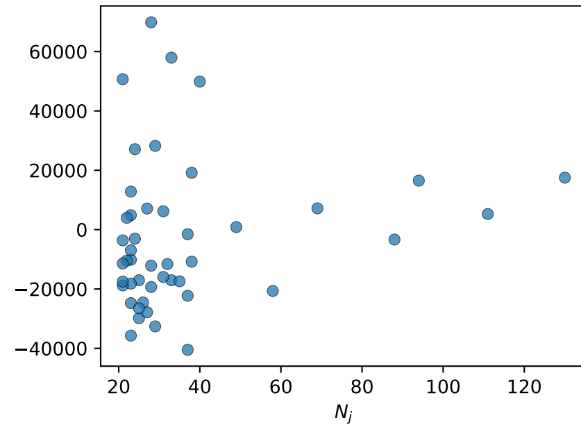
resid_mean Spearman \rho=0.19
