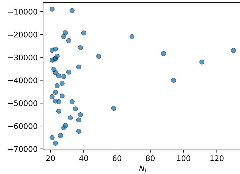
resid_q25 Spearman \rho=0.07
