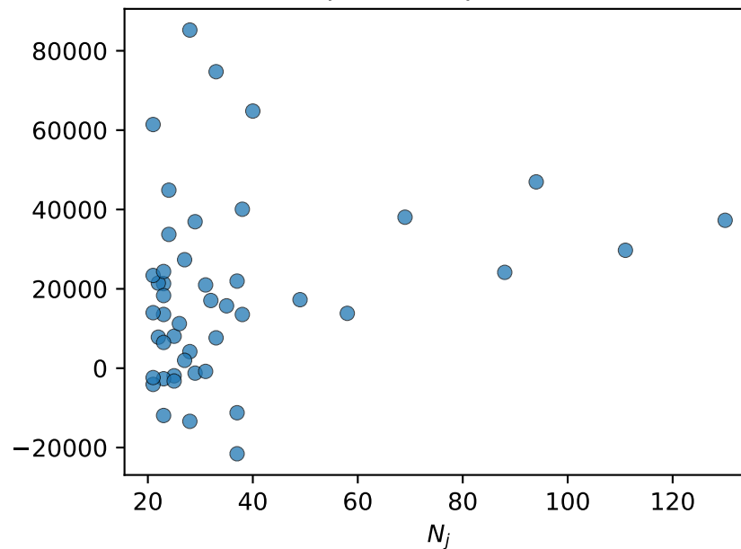
resid_q75 Spearman \rho=0.26
