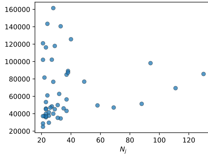
resid_sd Spearman \rho=0.31
