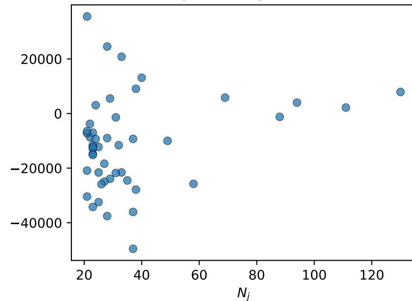
resid_median Spearman \rho=0.13
