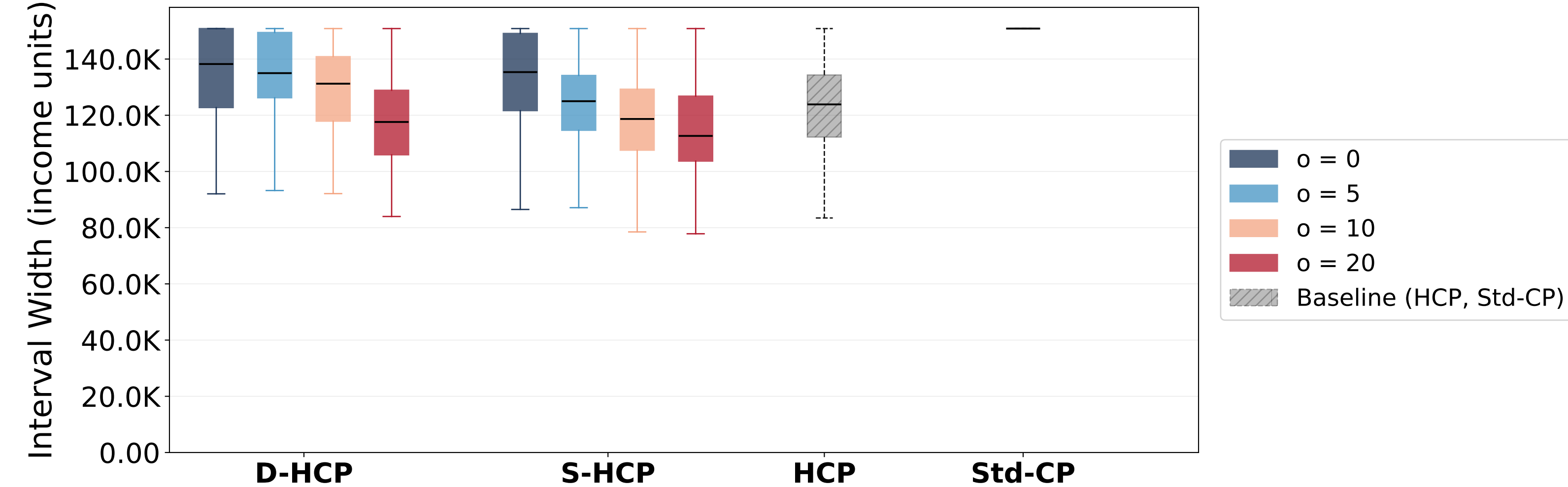
Interval Width (income units) - D-HCP / S-HCP vs HCP / Std-CP (90th pct clipped) - ACS (CA fixed PUMA groups, alpha=0.2)
