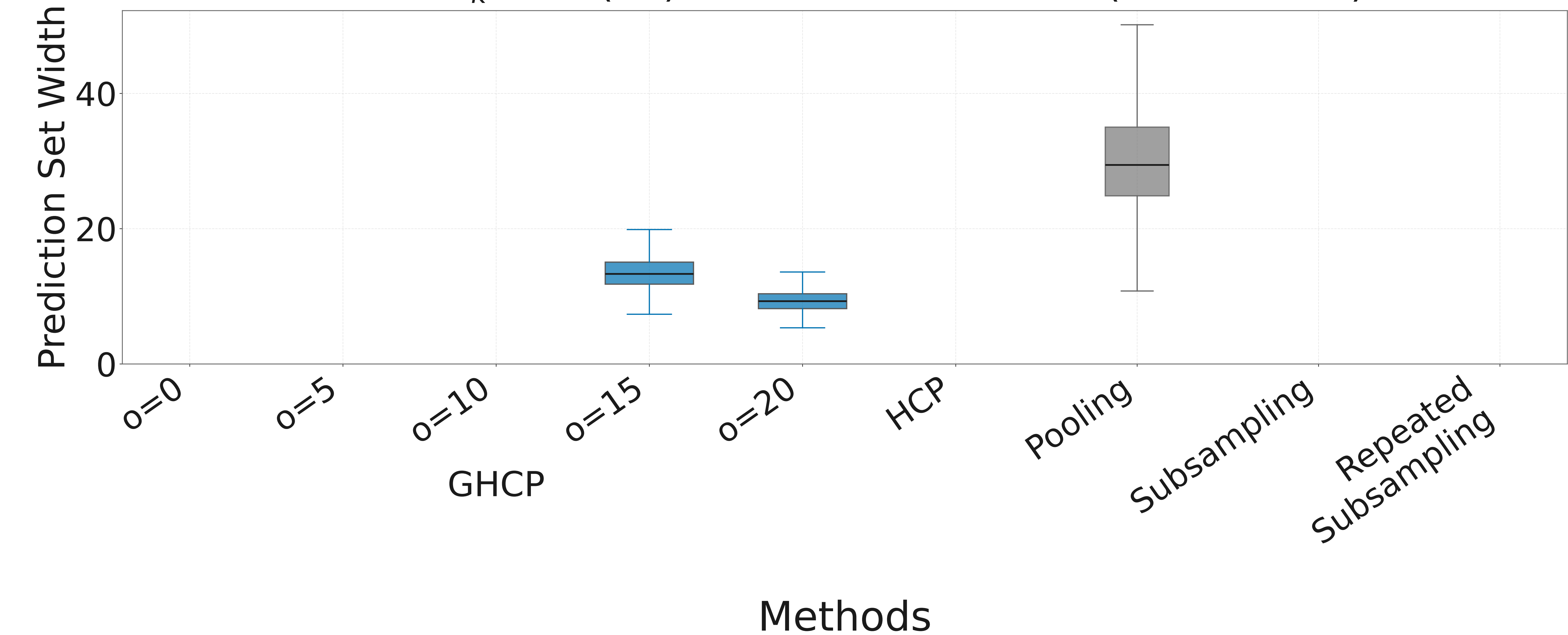
Fixed N_k = 21 (RF): Prediction set width (all methods)
