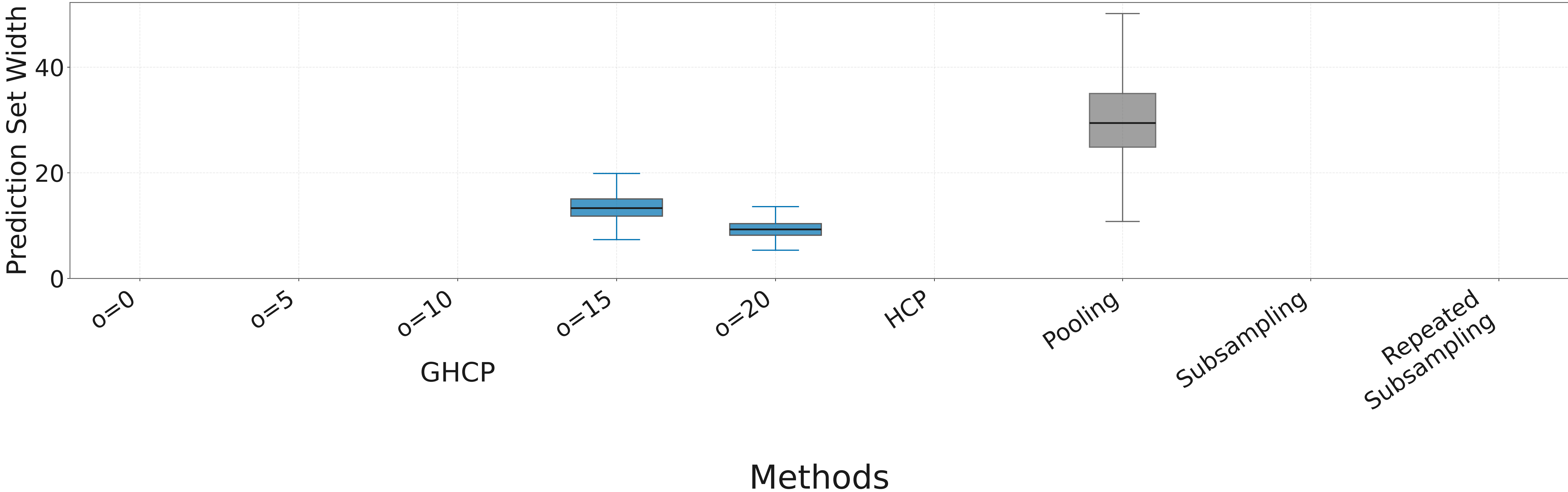
Fixed N_k = 21 (RF): Prediction set width (all methods)
