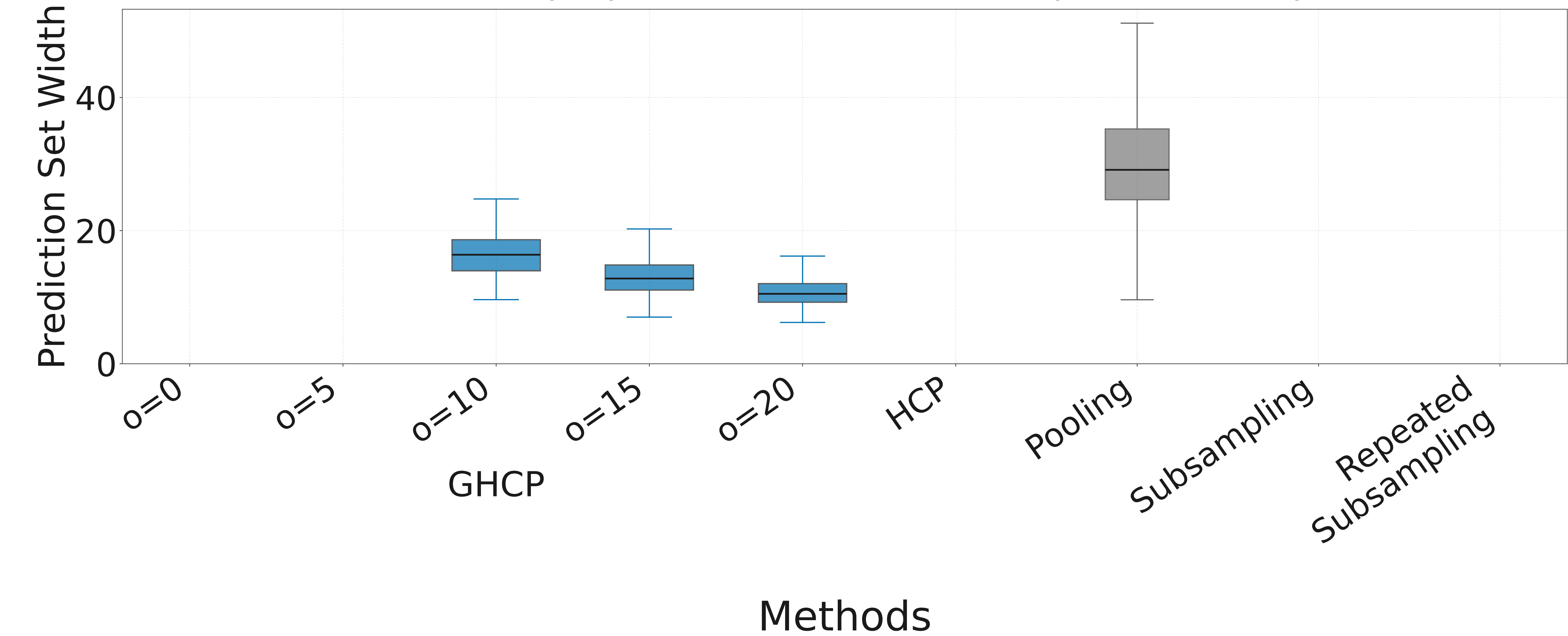
Poisson (RF): Prediction set width (all methods)
