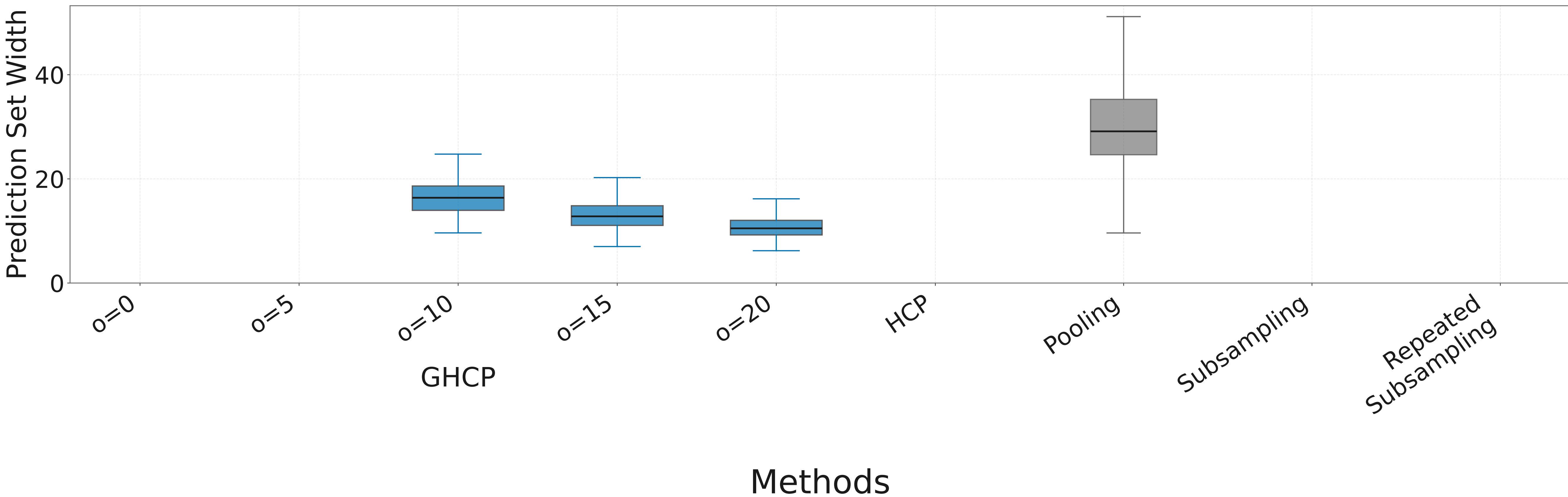
Poisson (RF): Prediction set width (all methods)
