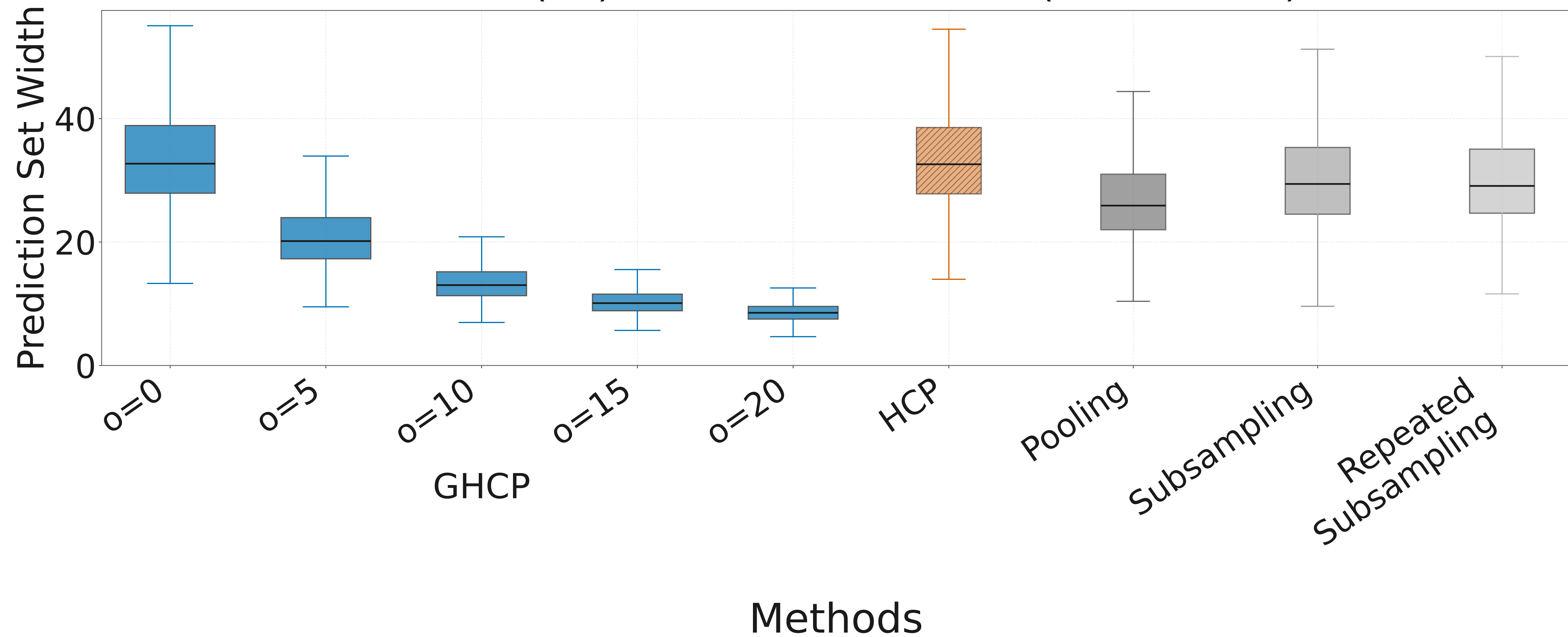
Poisson (RF): Prediction set width (all methods)
