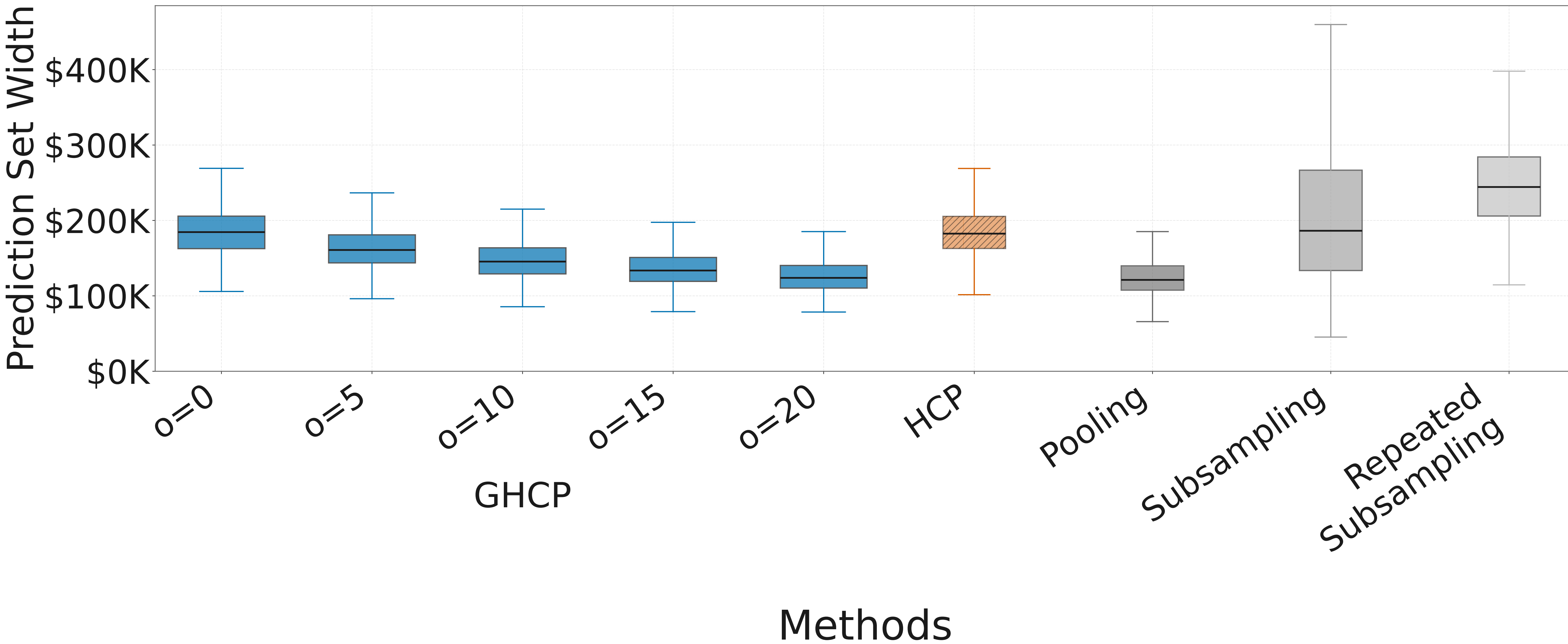
ACS (RF): Width
