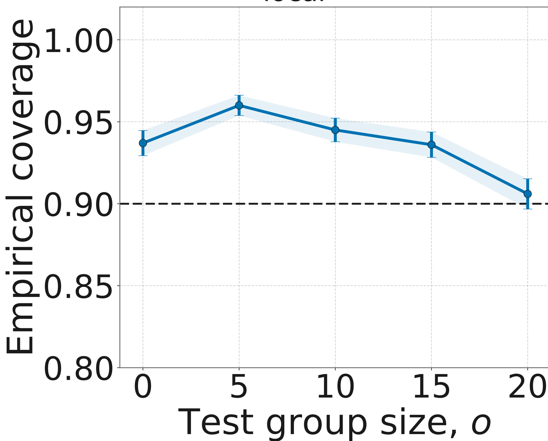
\lambda_{\text{local}} = 4/7
