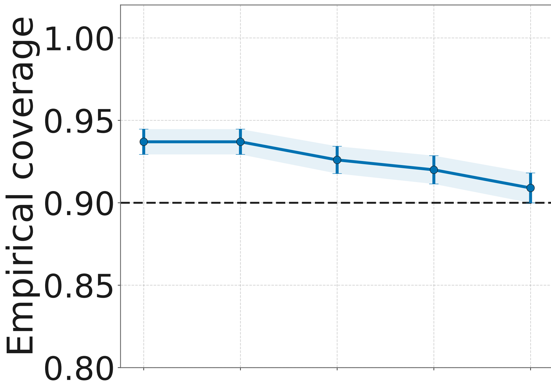
\lambda_{\text{local}} = 4/7
