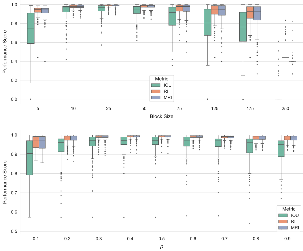
Figure 6: Effect on performance metrics (IOU and Rand Index) due to modification of the hyper-parameters of the WISER algorithm, namely block size (Top) and \rho (Bottom).
