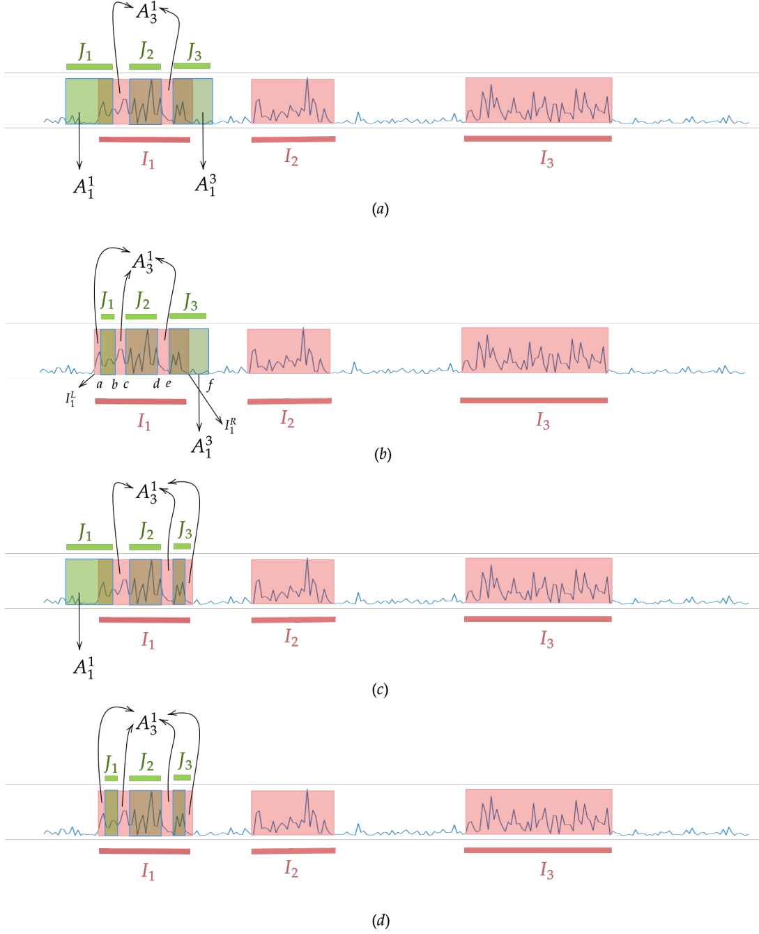
Figure 8: Representative cases for P_{(1,1,1,1,1)}^\emptyset in the proof of Theorem E.1.
