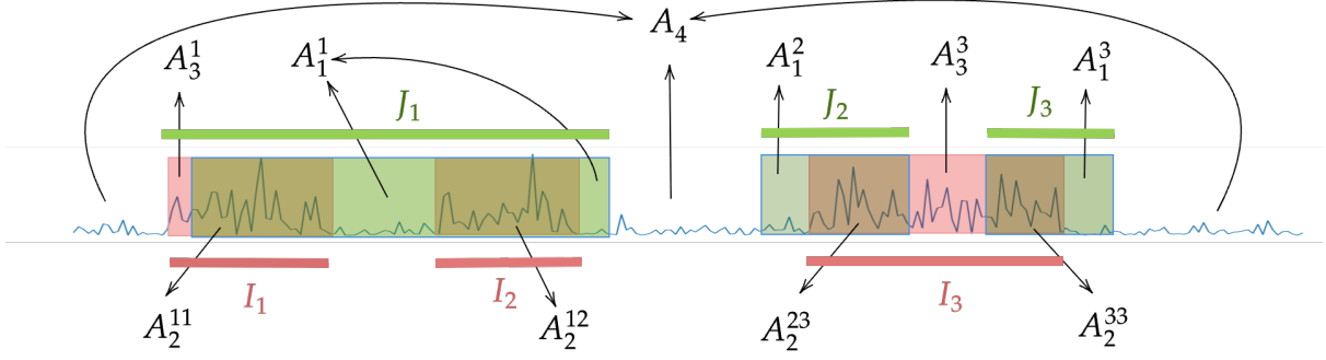
Figure 7: An instance of Case \mathcal{P}_{(1,2,3,3,3,3)}^{\emptyset} from Table 14.
