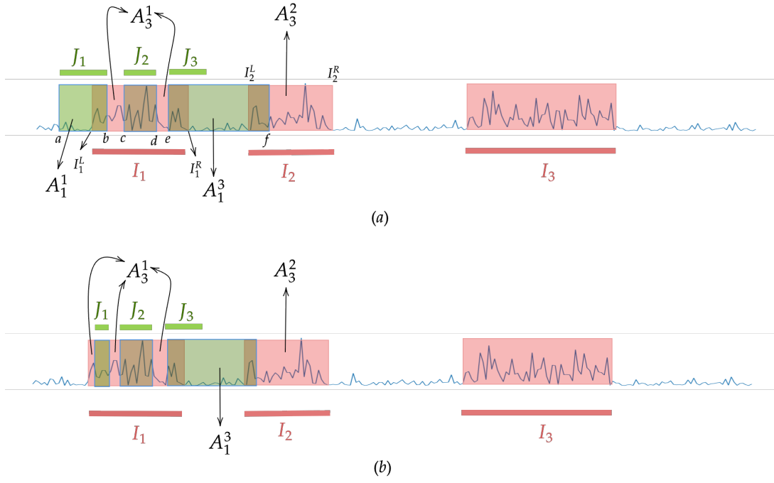
Figure 9: Representative cases for P_{(1,1,1,1,1,2)}^{\emptyset} in the proof of Theorem E.1.
