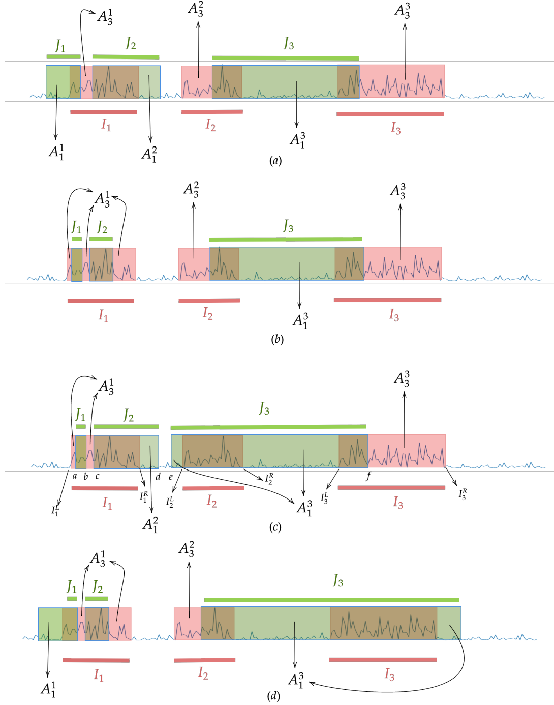
Figure 10: Some representative cases for P_{(1,1,1,1,2,3)}^\emptyset , used in the proof of Theorem E.1. For example, the interactions between (I_1, J_1) , (I_1, J_2) , (I_2, J_3) and (I_3, J_3) , are of the types (a) (\mathcal{P}_4, \mathcal{P}_5, \mathcal{P}_5, \mathcal{P}_4) , (b) (\mathcal{P}_1, \mathcal{P}_1, \mathcal{P}_5, \mathcal{P}_4) , (c) (\mathcal{P}_1, \mathcal{P}_5, \mathcal{P}_2, \mathcal{P}_4) , and (d) (\mathcal{P}_4, \mathcal{P}_1, \mathcal{P}_5, \mathcal{P}_2) respectively.
