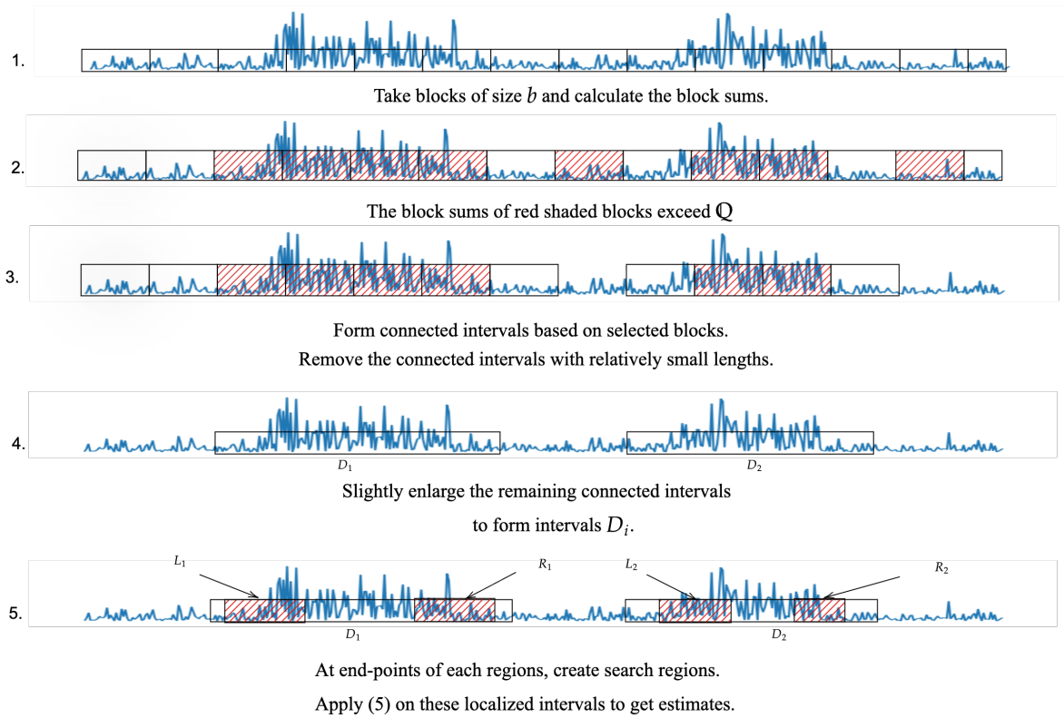
Figure 2: WISER in action with key steps.
