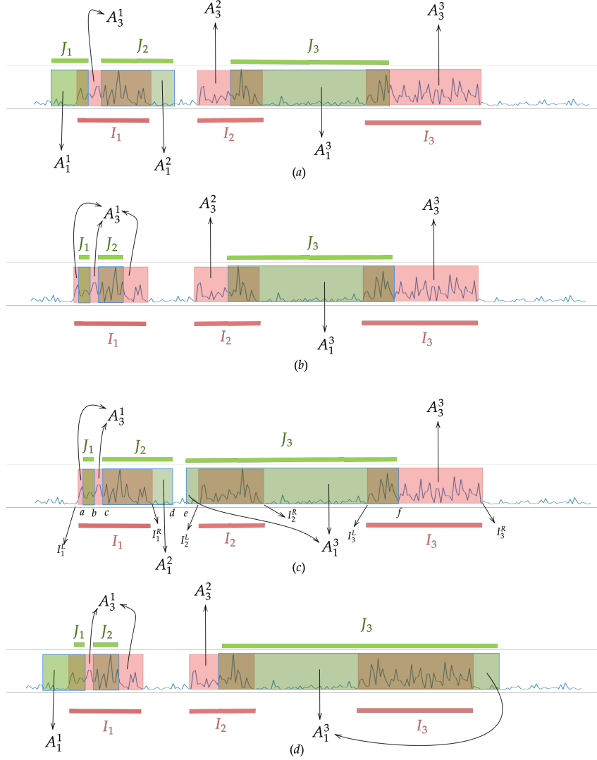
Figure 11: Some representative cases for P_{(1,1,1,1,2,3)}^\partial , used in the proof of Theorem C.1. For example, the interactions between (I_1, J_1) , (I_1, J_2) , (I_2, J_3) and (I_3, J_3) , are of the types (a) (\mathcal{P}_4, \mathcal{P}_5, \mathcal{P}_5, \mathcal{P}_4) , (b) (\mathcal{P}_1, \mathcal{P}_1, \mathcal{P}_5, \mathcal{P}_4) , (c) (\mathcal{P}_1, \mathcal{P}_5, \mathcal{P}_2, \mathcal{P}_4) , and (d) (\mathcal{P}_4, \mathcal{P}_1, \mathcal{P}_5, \mathcal{P}_2) respectively.
