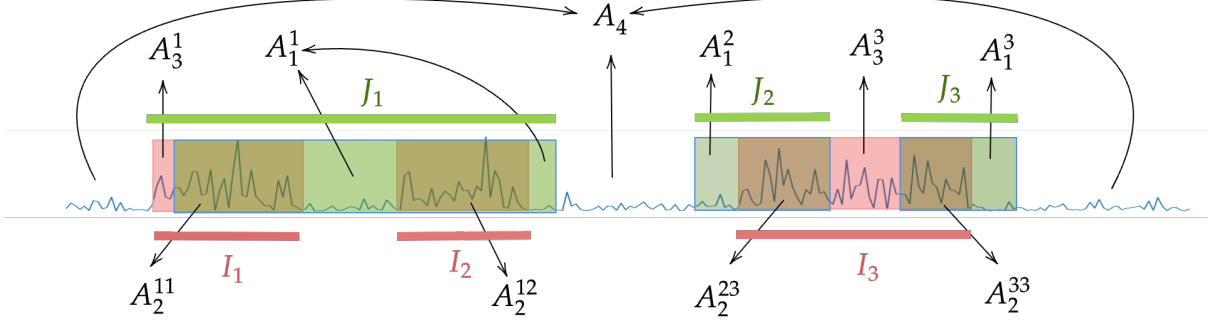
Figure 8: An instance of Case \mathcal{P}_{(1,2,3,3,3,3)}^{\emptyset} from Table 17.
