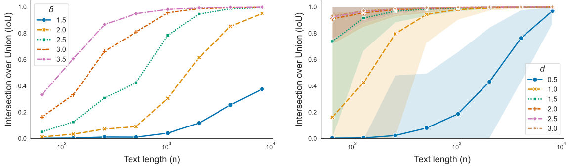
Figure 4: IOU of WISER algorithm across different length texts. (Left) for different levels of \delta in Red-green watermarking; (Right) for different levels of d as in Assumption 2.2 for Gumbel watermarking scheme. X-axis is on a log scale for both plots.
