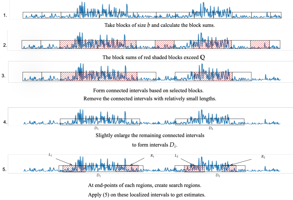
Figure 2: WISER in action with key steps.
