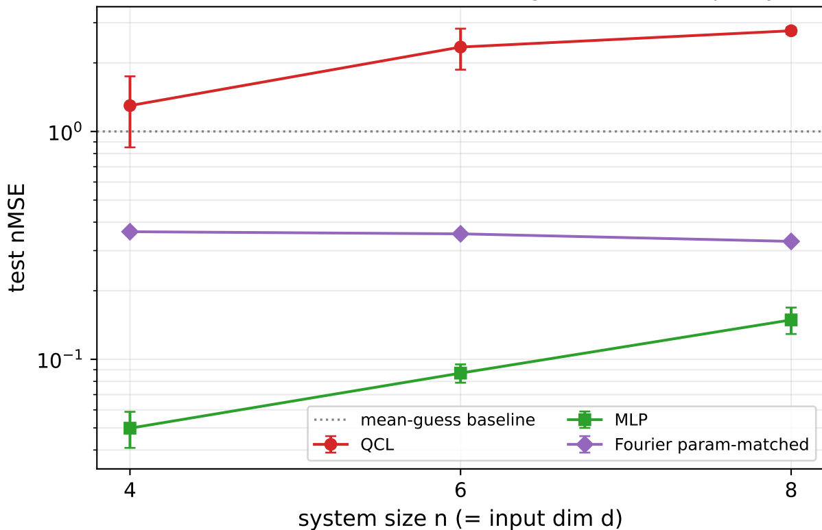
Disordered Hubbard ( d = n ) — target: double occupancy
