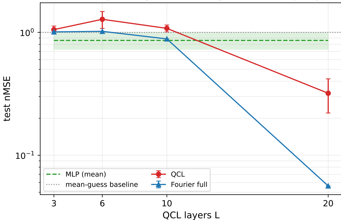
Hubbard quench dynamics — target: double occupancy
