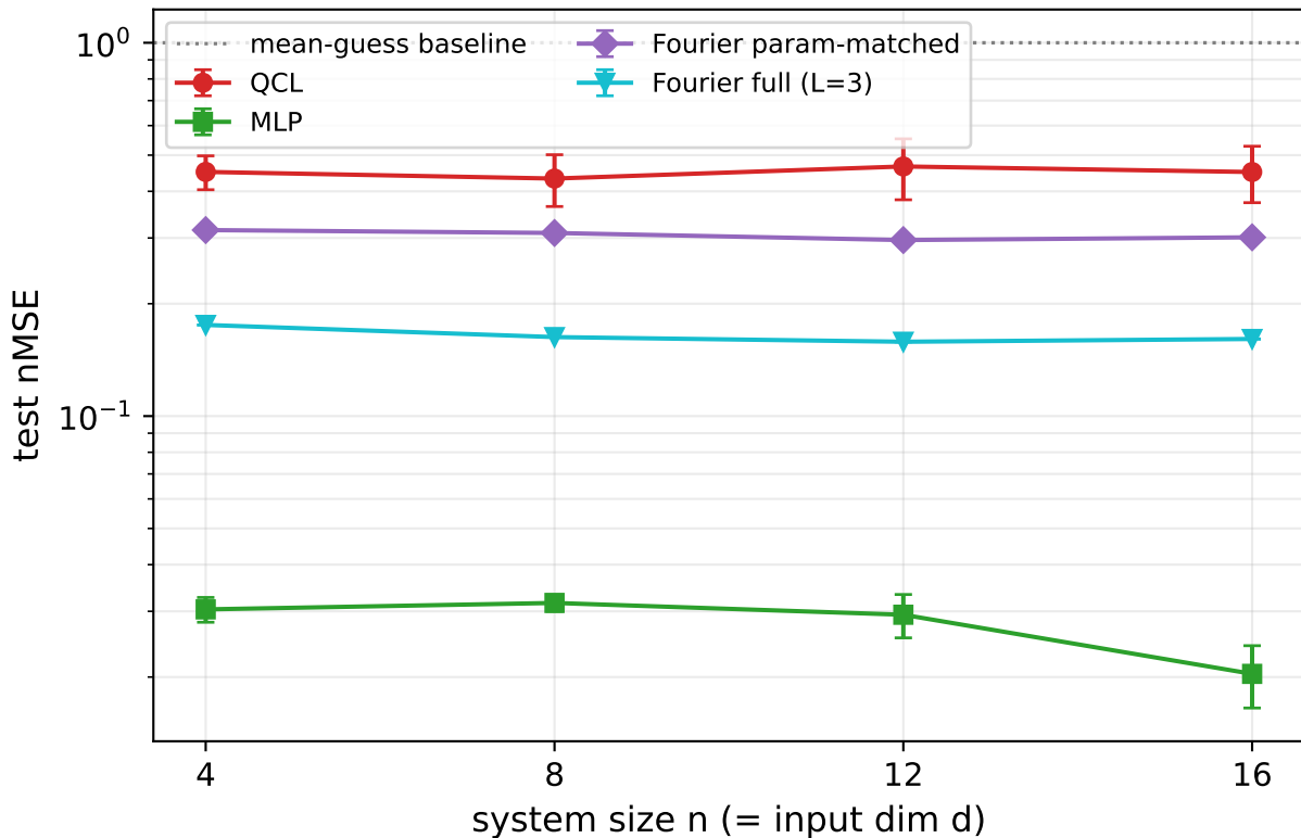
Static XY — target: entanglement entropy
